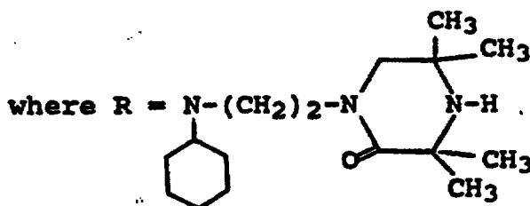
oxo-piperazinyll ring
