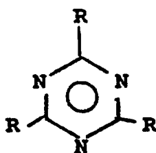
triazine ring
