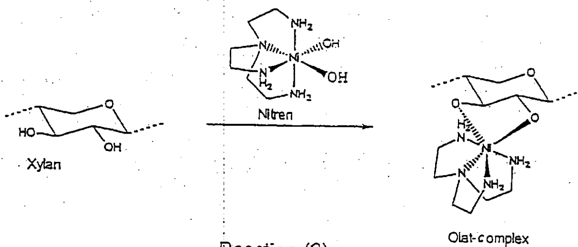
Reaction (2)
