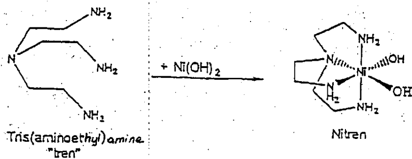
Reaction (1)
