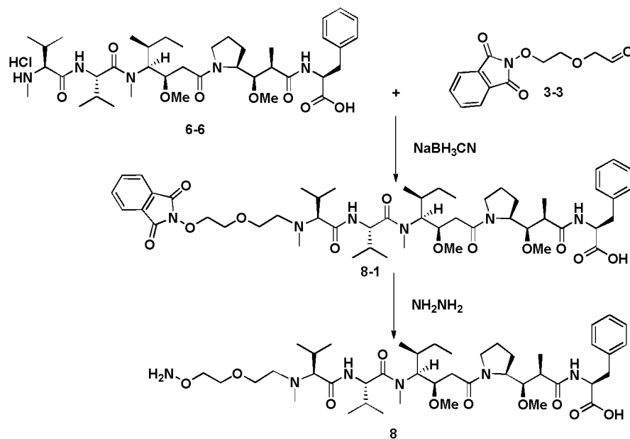
Scheme 8
