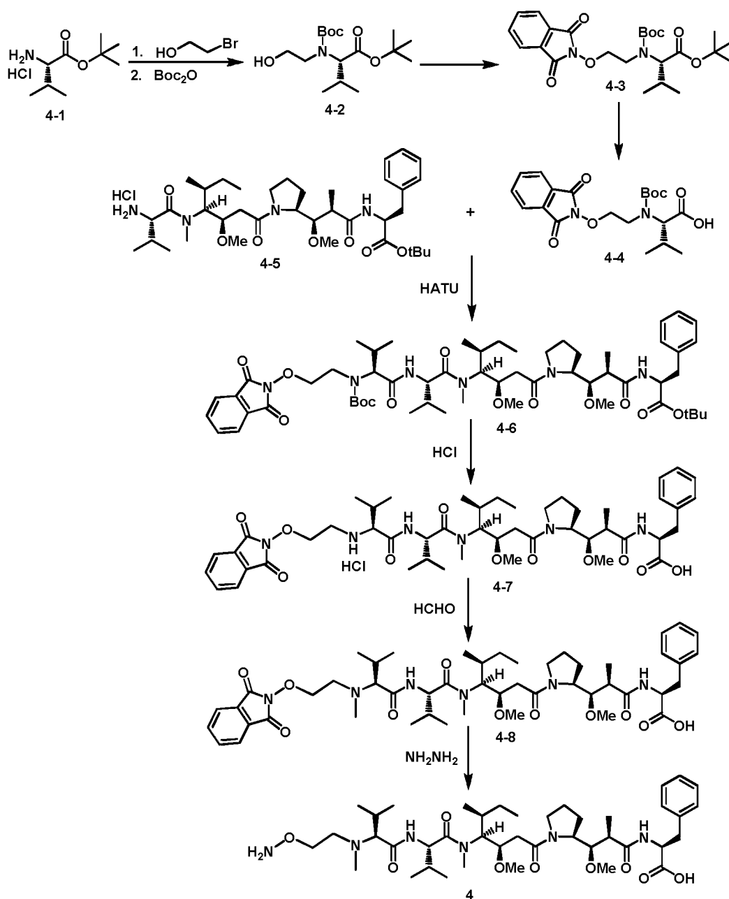
Scheme 4
