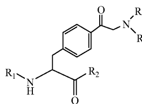
(XXXXXXIII),
