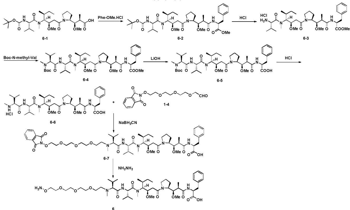
Scheme 6
