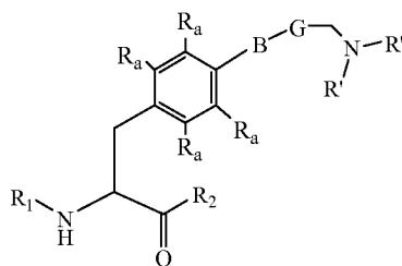
(XXXXXXIII),
