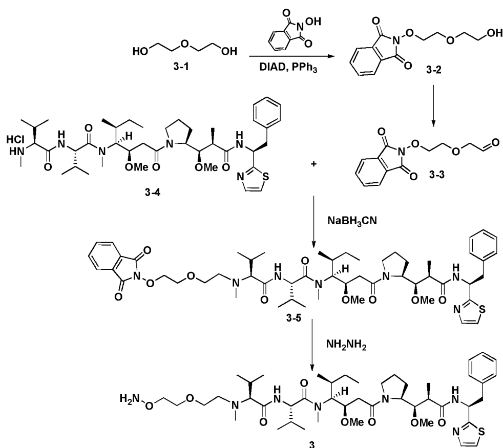
Scheme 3
