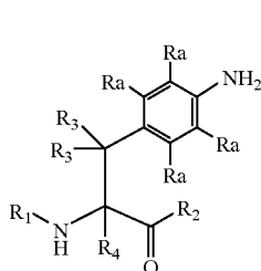
(XXXXXXVI),
