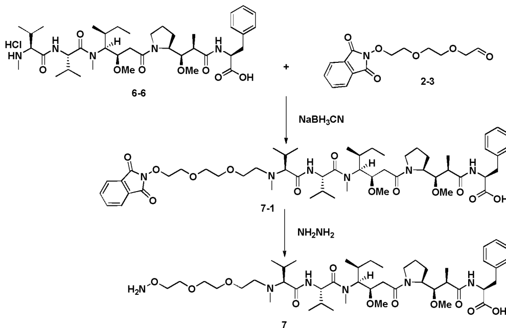
Scheme 7
