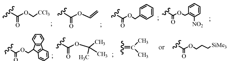
(XXXXXXVI),
