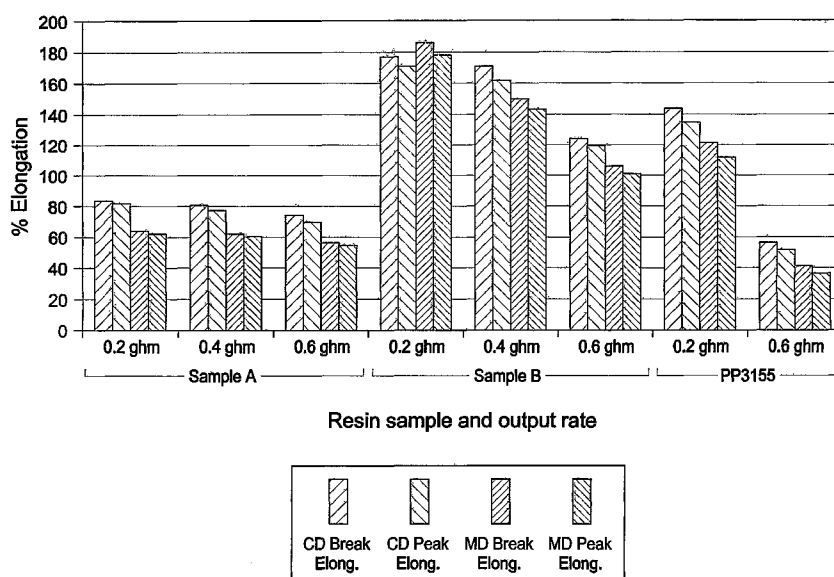
Comparison of Melt Blown Fabric Elongation
