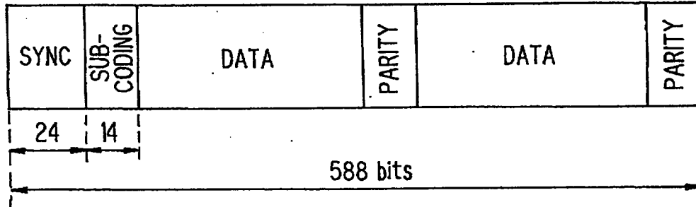
FRAME STRUCTURE
