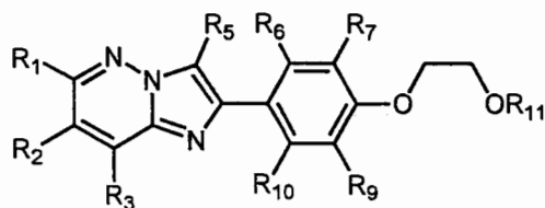
Formula (V);
