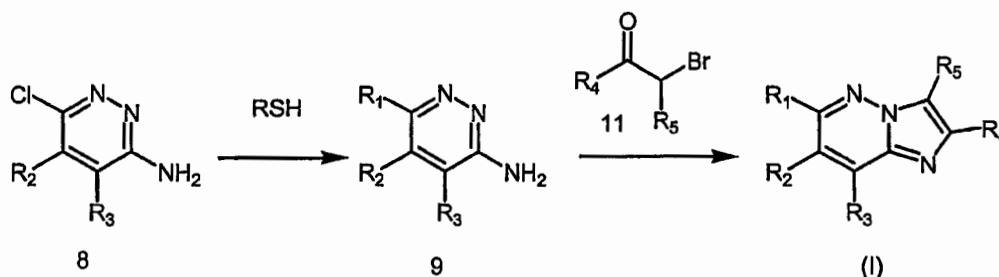
Scheme 4
