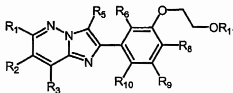
Formula (VI)
