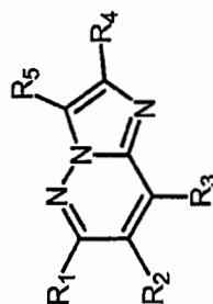
Formula (I)
