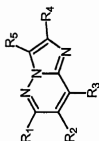
Formula (I)
