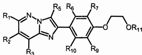
Formula (V)
