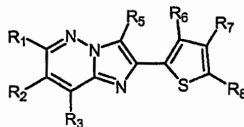
Formula (IV)
