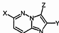
Formula A
