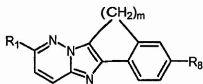
Formula (VI)
