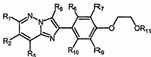
Formula (V)
