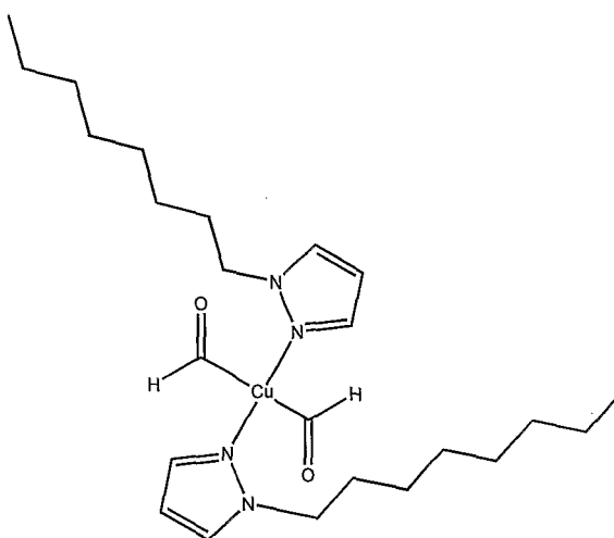
Structure 2. 1-octylpyrazole copper formate complex
