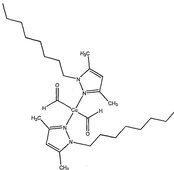
Structure 1. 1-octyl-3,5-dimethylpyrazole copper formate complex
