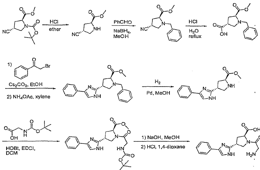
Scheme 12
