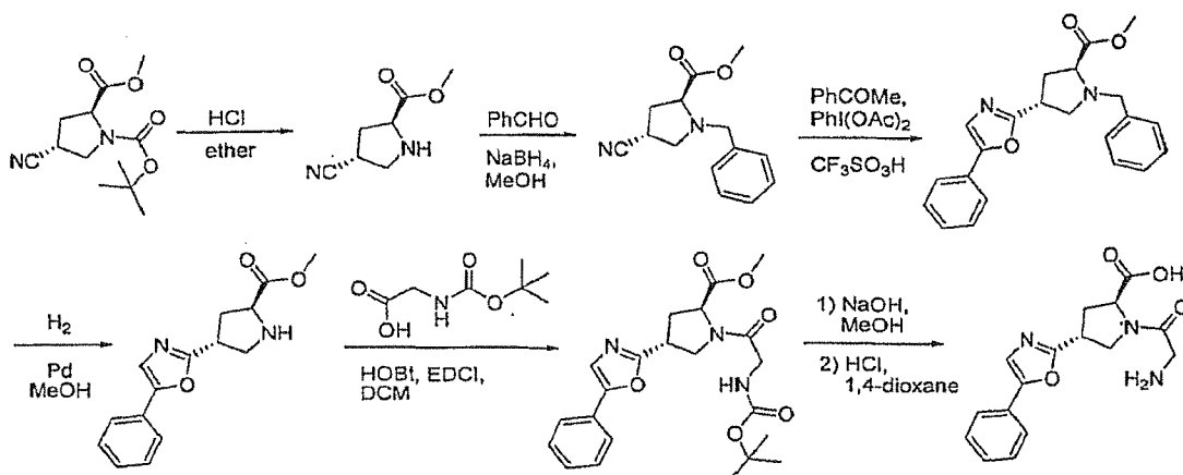
Scheme 11
