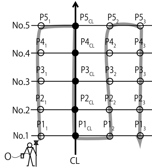
Route direction
