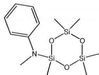
2-phenylmethylamino-2,4,4,6,6-pentamethylcyclotrisiloxane
