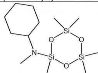
2-cyclohexylmethylamino-2,4,4,6,6-pentamethylcyclotrisiloxane
