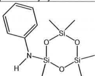
2-phenylamino-2,4,4,6,6-pentamethylcyclotrisiloxane
