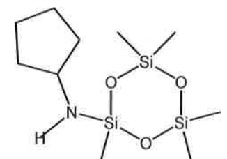
2-cyclopentylamino-2,4,4,6,6-pentamethylcyclotrisiloxane
