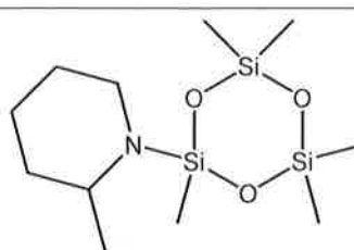
2-(2-methylpiperidino)-2,4,4,6,6-pentamethylcyclotrisiloxane
