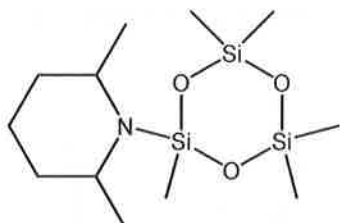
2-(2,6-dimethylpiperidino)-2,4,4,6,6-pentamethylcyclotrisiloxane
