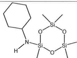
2-cyclohexylamino-2,4,4,6,6-pentamethylcyclotrisiloxane
