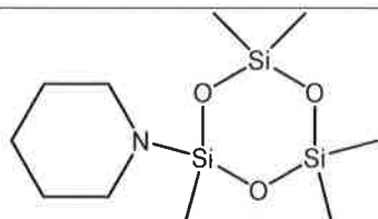
2-piperidino-2,4,4,6,6-pentamethylcyclotrisiloxane
