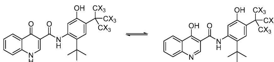
Tautomers of Formula 9
