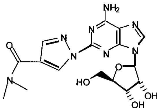
(1-{9-[(4S,2R,3R,5R)-3,4-dihydroxy-5-(hydroxymethyl)oxolan-2-yl]-6-aminopurin-2-yl}pyrazol-4-yl)-N,N-dimethylcarboxamide (18)
