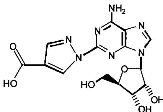
1-{9-[(4S,2R,3R,5R)-3,4-dihydroxy-5-(hydroxymethyl)oxolan-2-yl]-6-aminopurin-2-yl}pyrazole-4-carboxylic acid (17)
