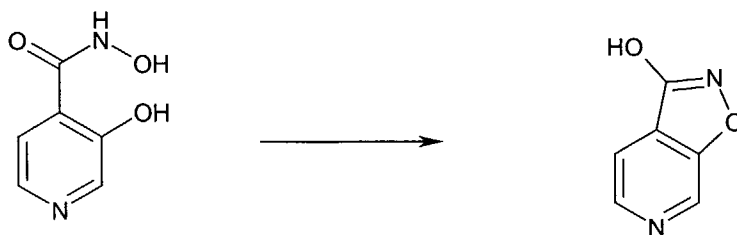
Isoxazolo[5,4-c]pyridin-3-ol (HIP)
