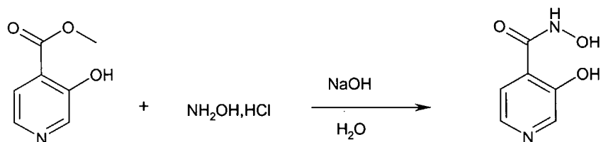
3,N-Dihydroxy-isonicotinamide
