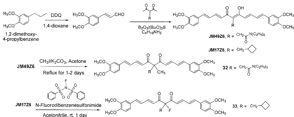
Scheme 20
