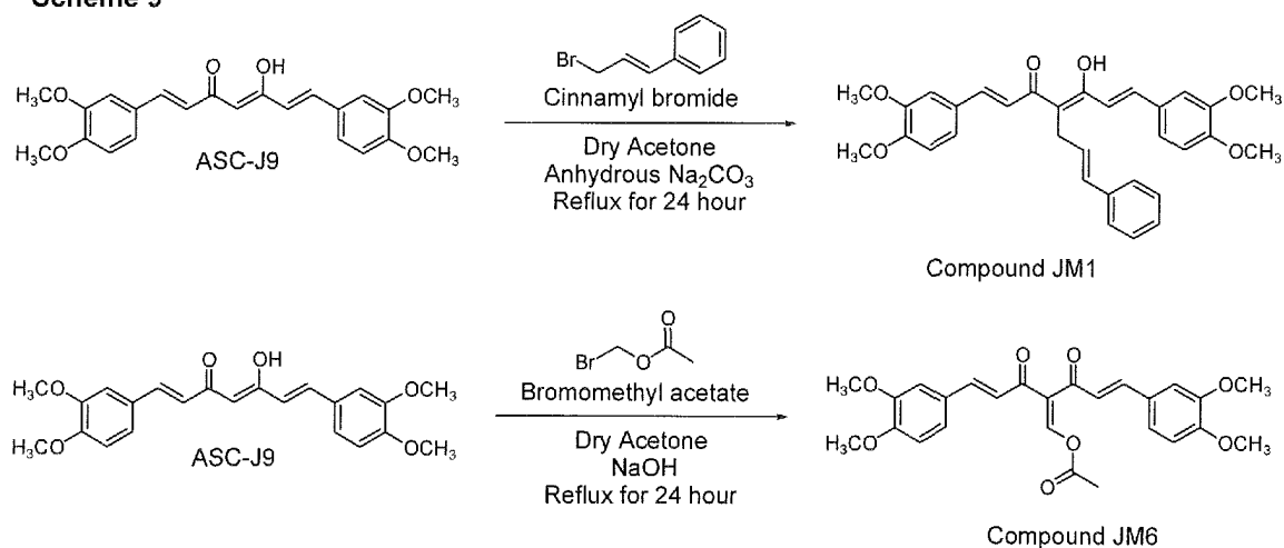
Scheme 9
