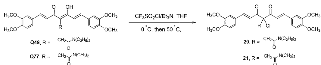
Scheme 17
