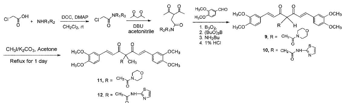
Scheme 15
