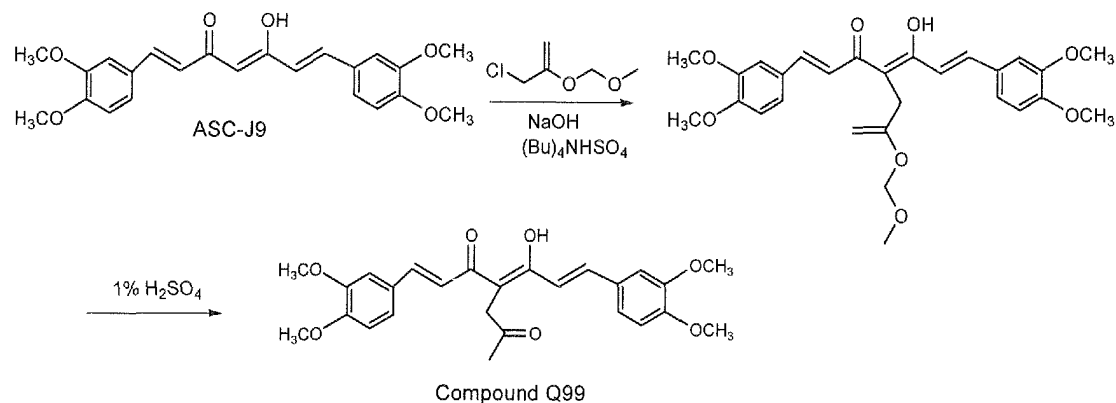
Scheme 6
