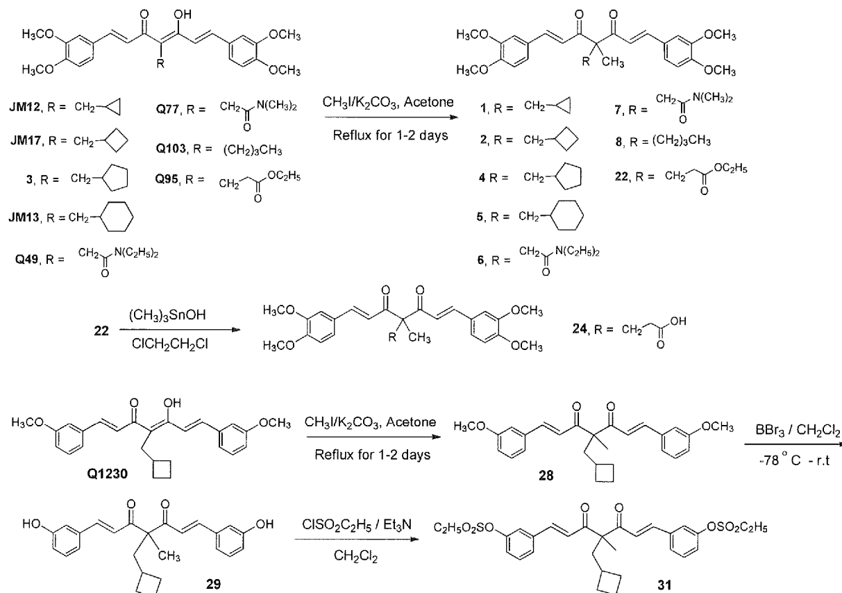
Scheme 14
