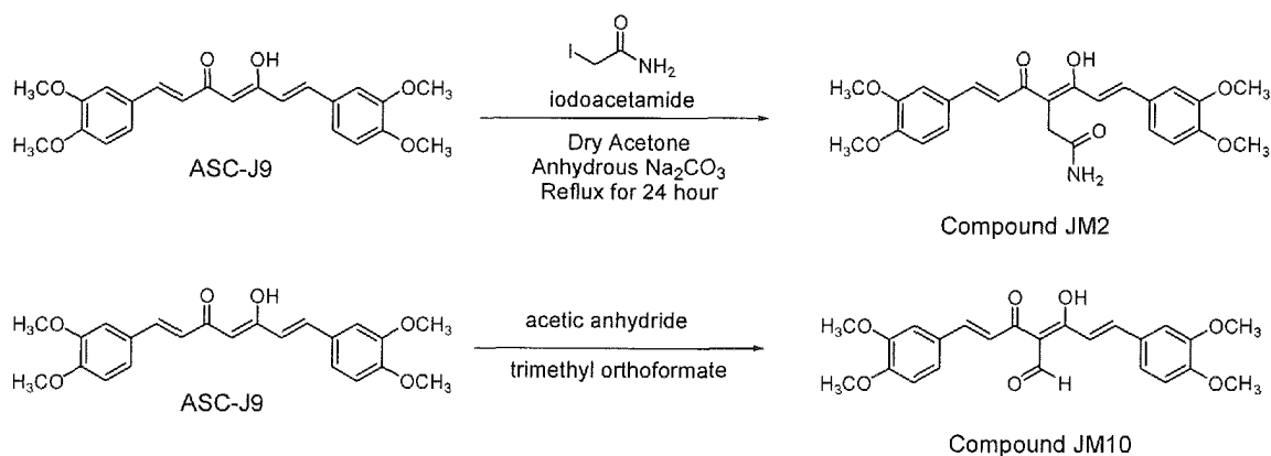
Scheme 7
