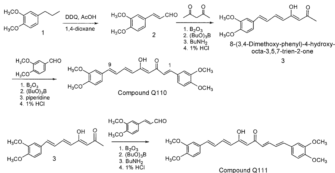
Scheme 13
