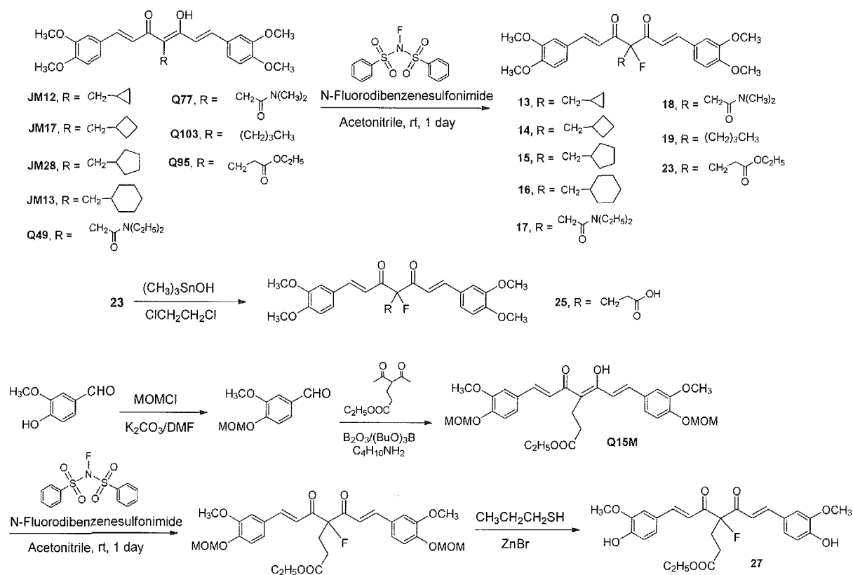
Scheme 16
