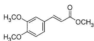
Monomer-1
