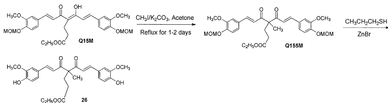
Scheme 18
