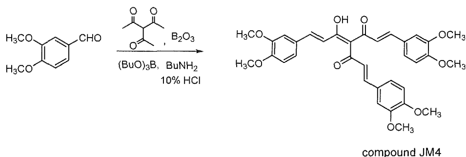
Scheme 11
