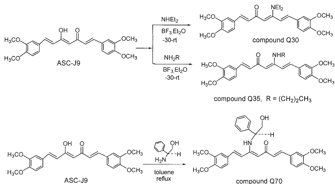
Scheme 5
