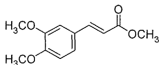
Monomer-1
