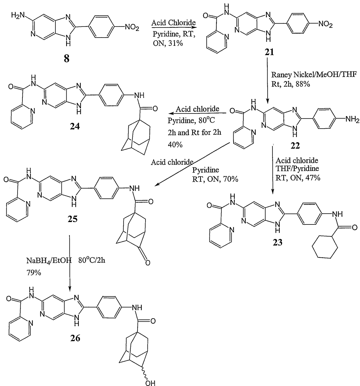
Scheme 41
