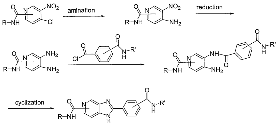
Synthetic Scheme 15
