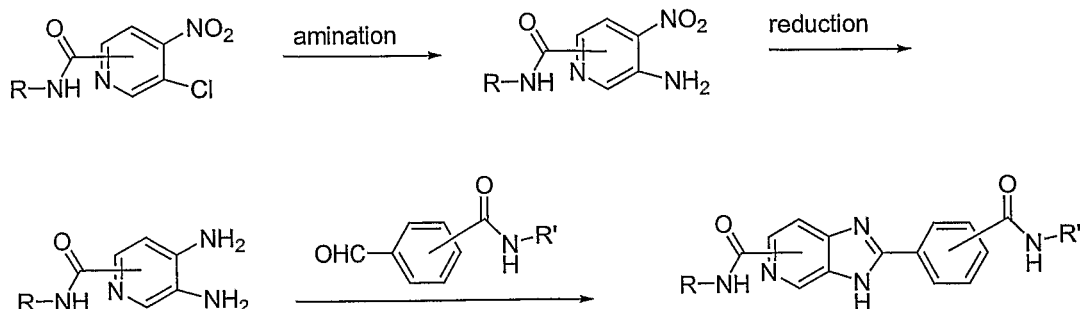
Synthetic Scheme 14
