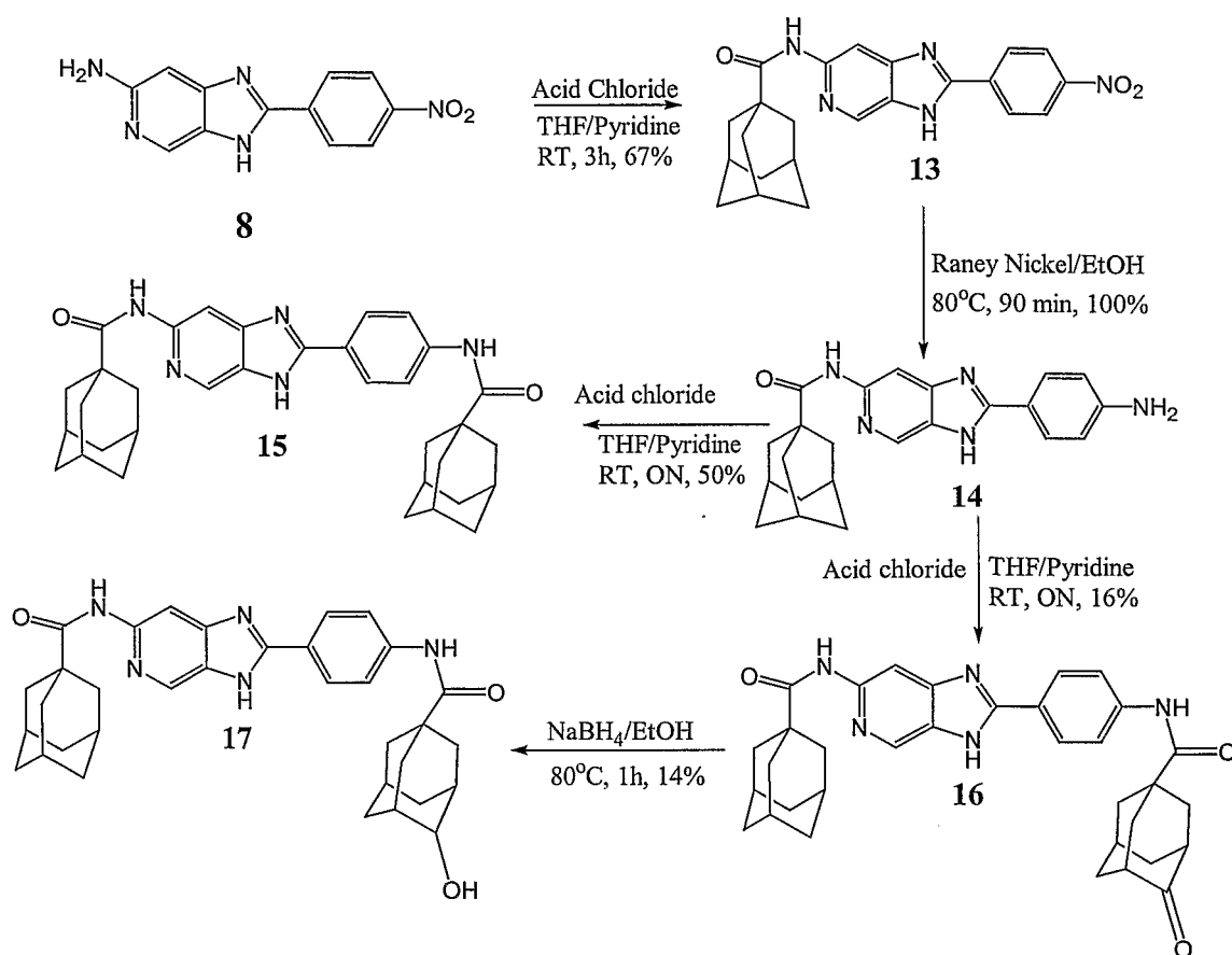
Scheme 39
