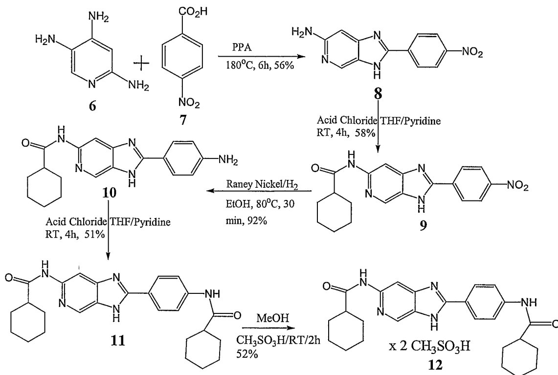
Scheme 38
