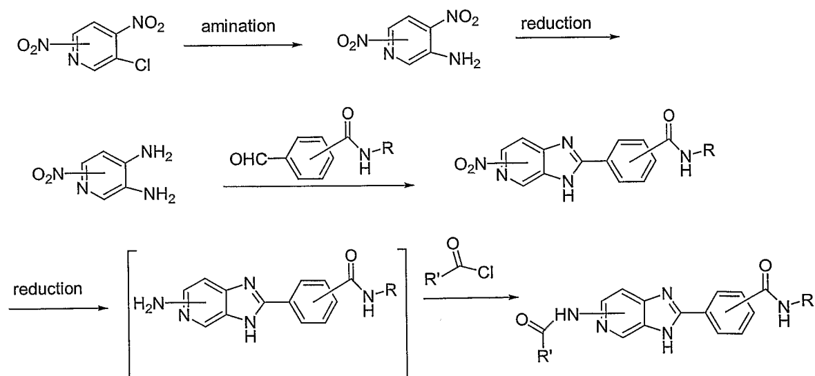
Synthetic Scheme 22
