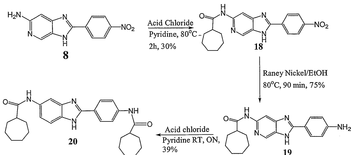
Scheme 40
