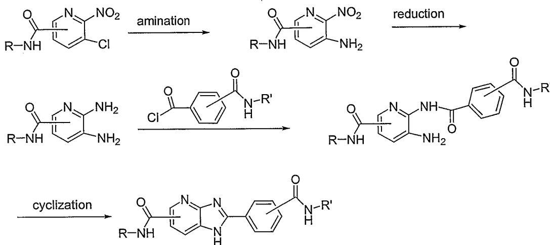
Synthetic Scheme 17
