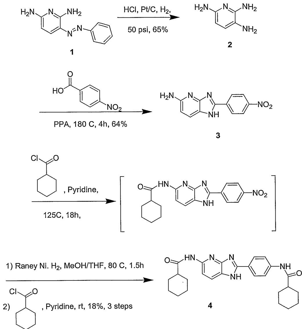
Scheme 43
