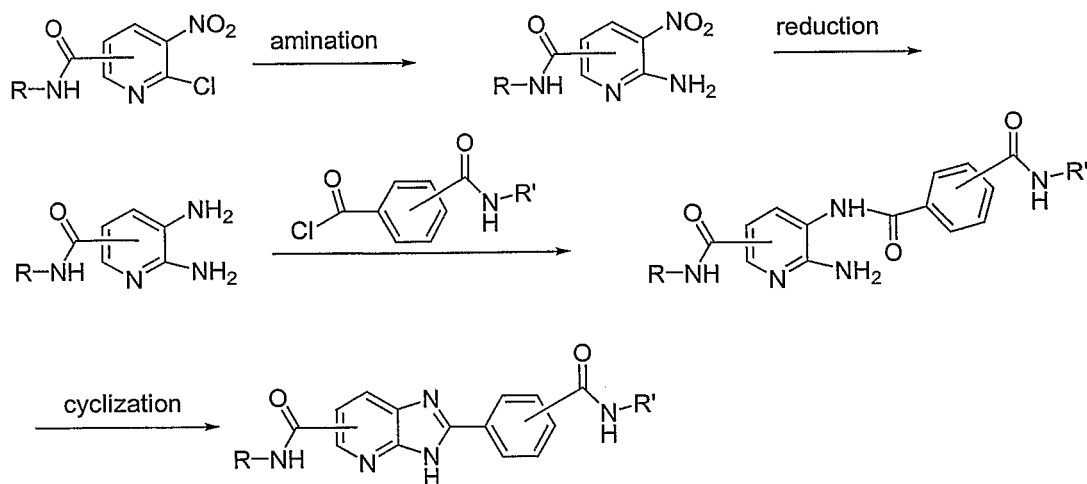
Synthetic Scheme 11
