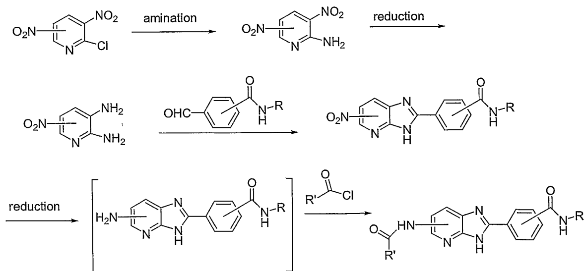
Synthetic Scheme 20
