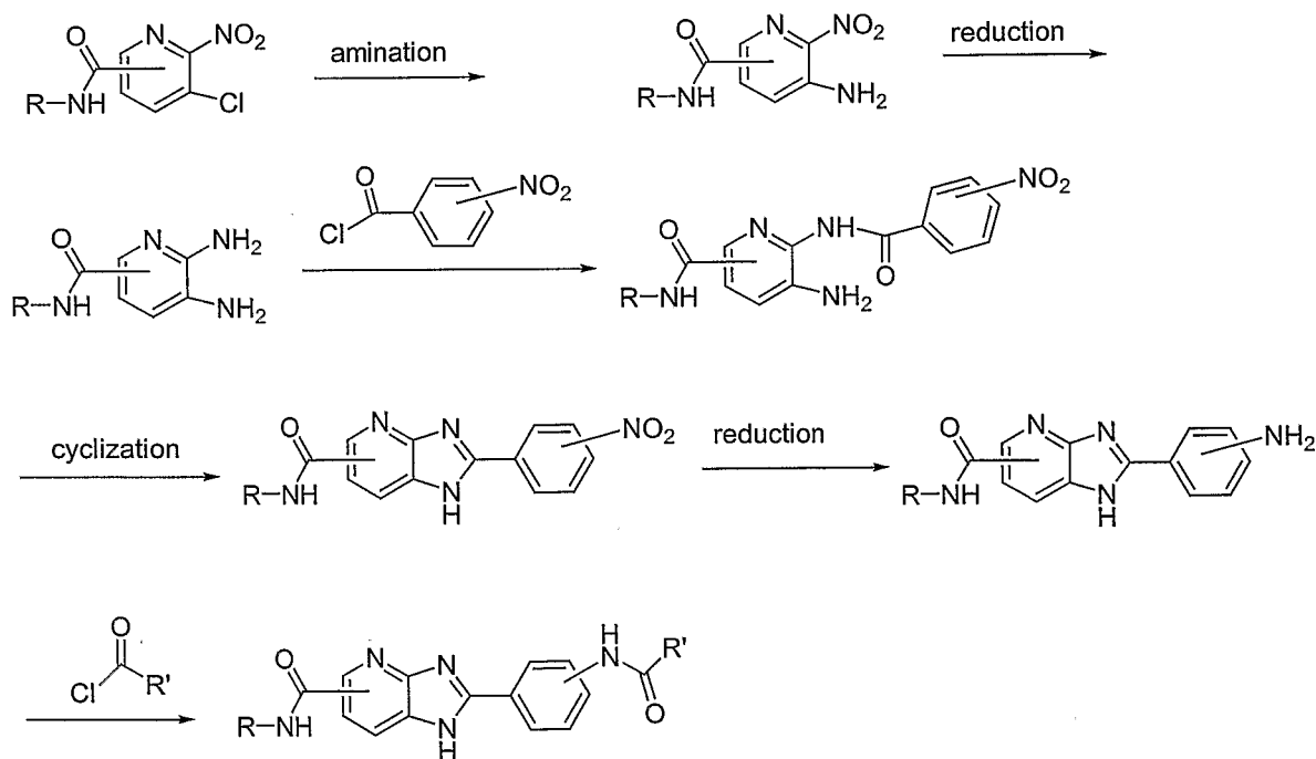
Synthetic Scheme 7
