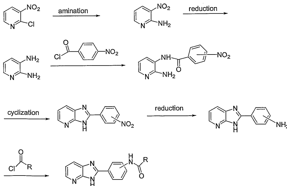
Synthetic Scheme 9
