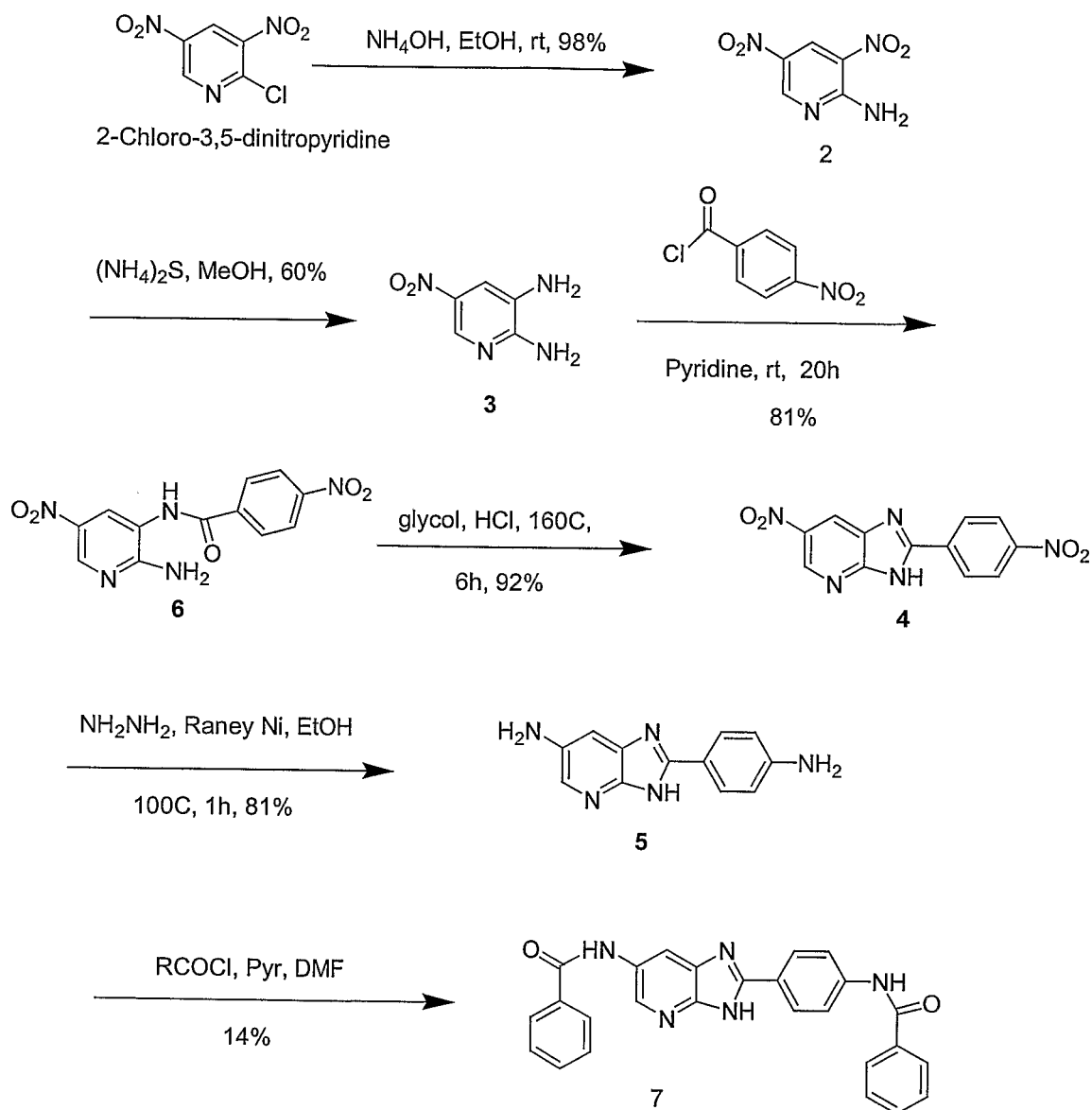
Scheme 36
