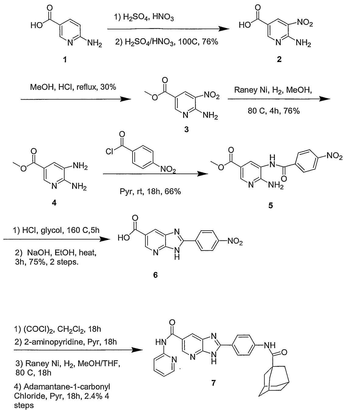
Scheme 42
