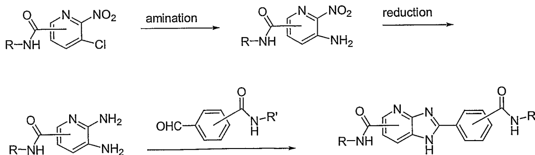
Synthetic Scheme 18
