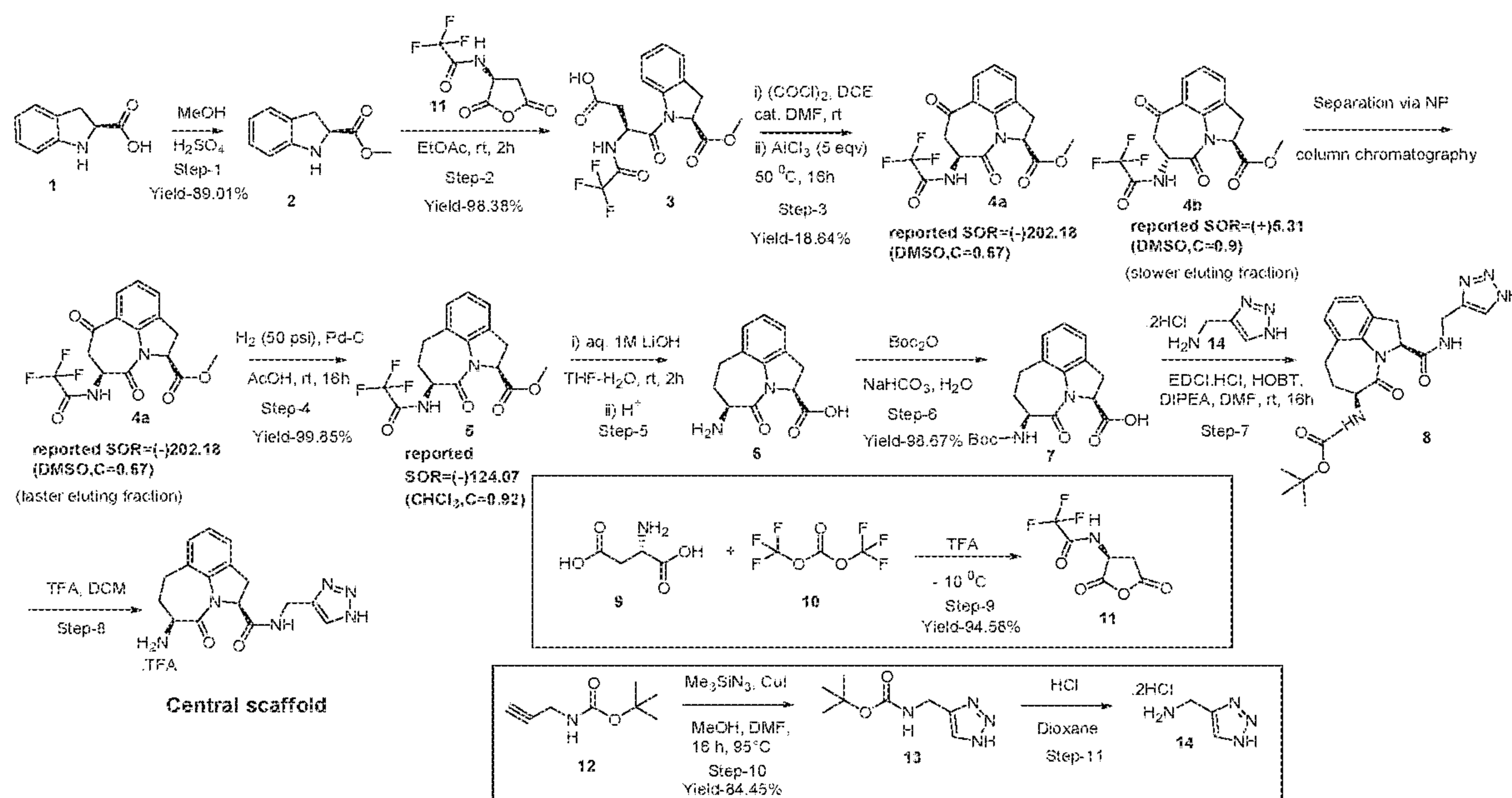
Scheme-1 [Synthesis of central scaffold, Reference-WO/9501353A1]:
