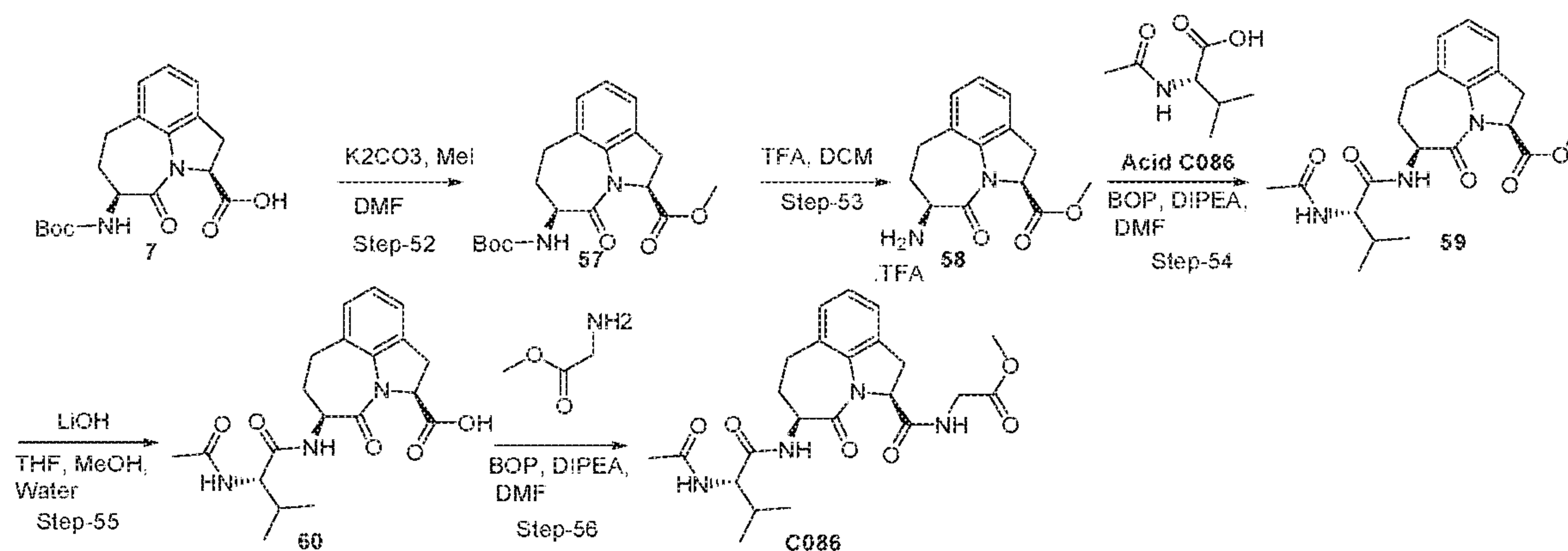
Scheme-13 [Synthesis of C086]
