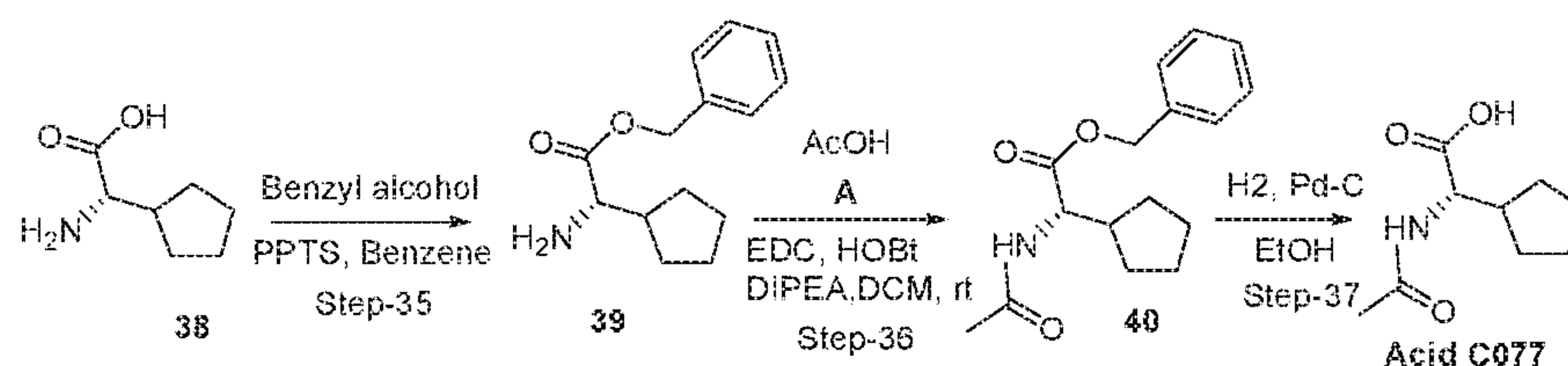
Scheme-9 [Synthesis of Acid C077]:
