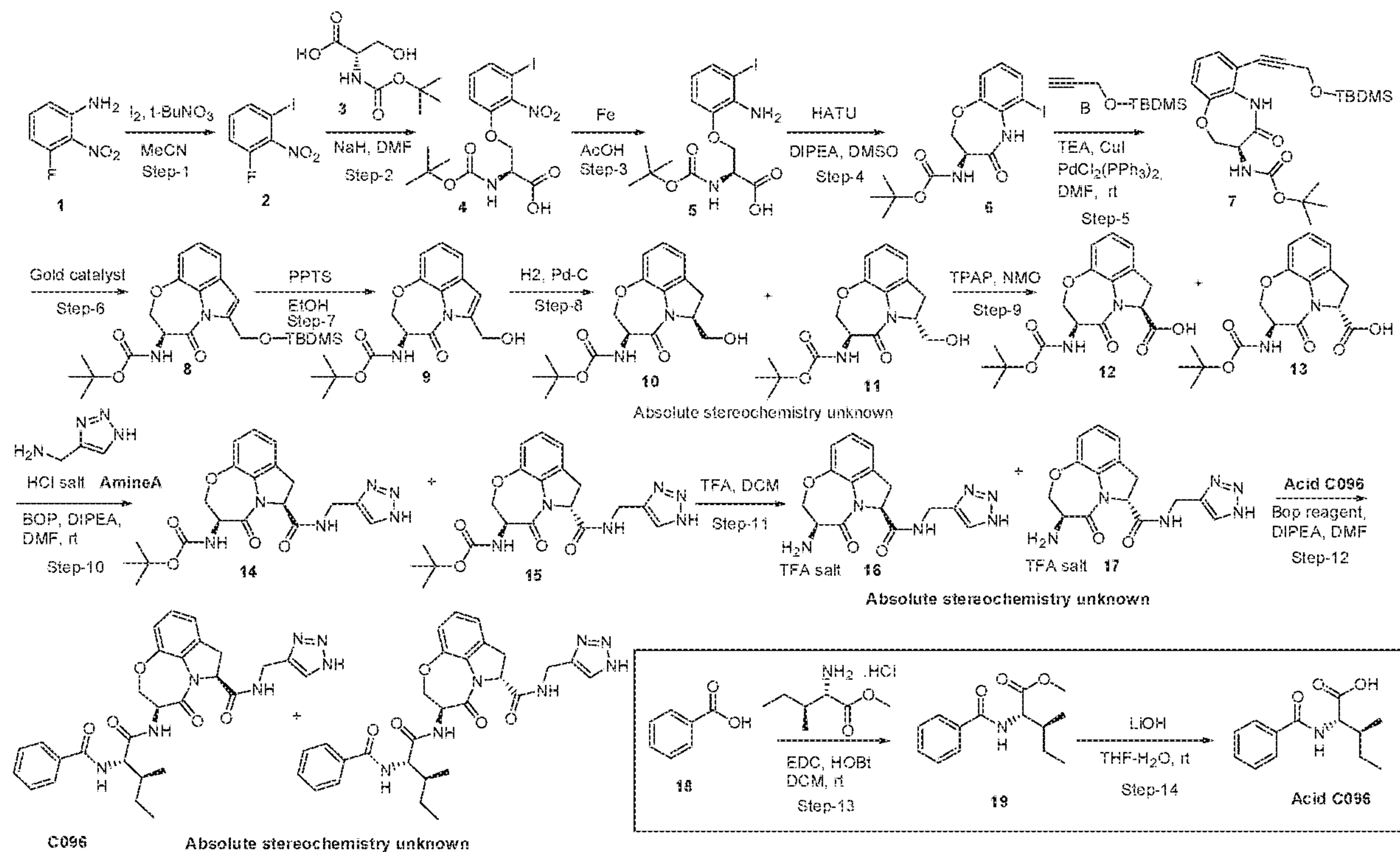
Scheme-20: Synthesis of oxygen-containing compounds
