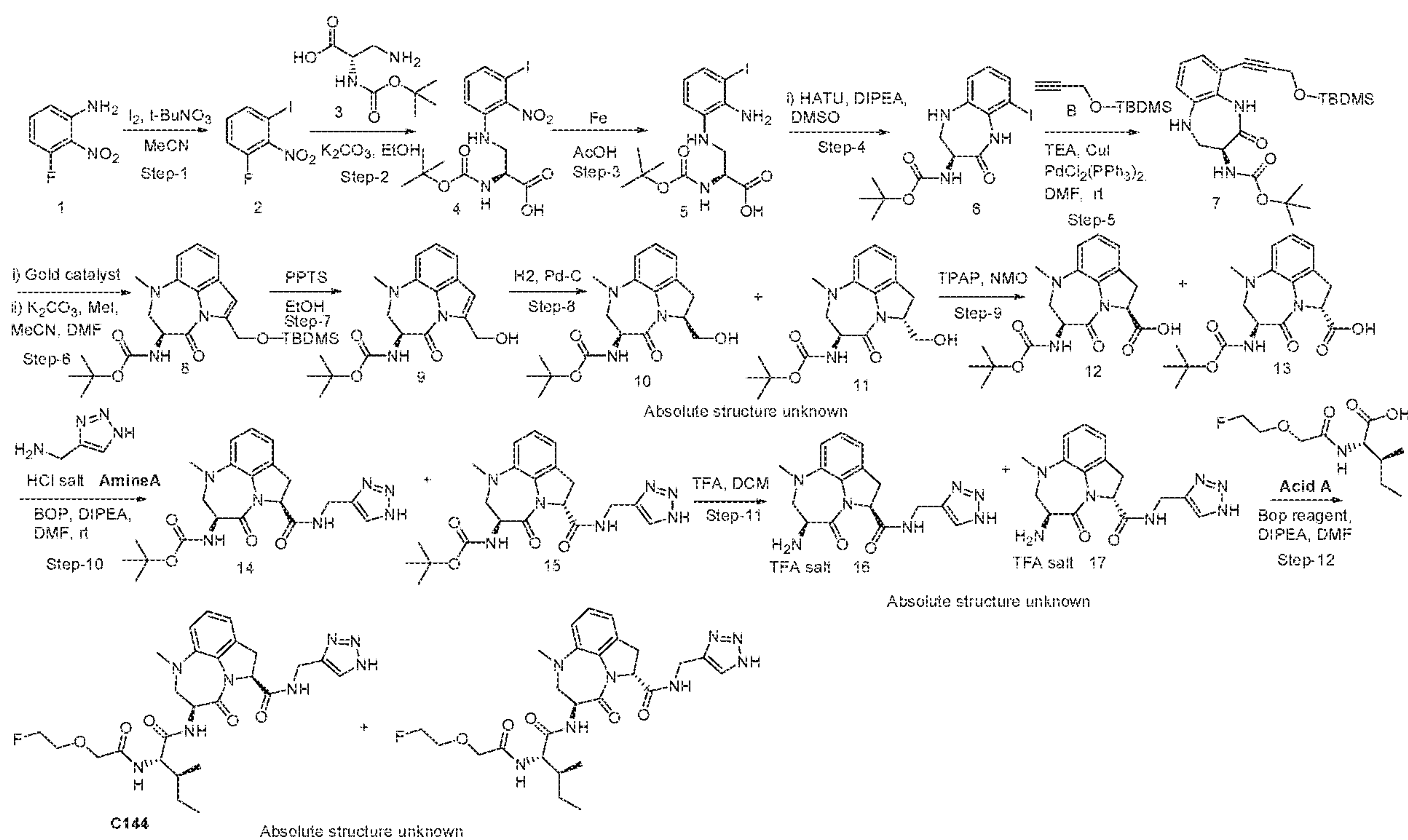
Scheme-25 [Synthesis of C144]:
