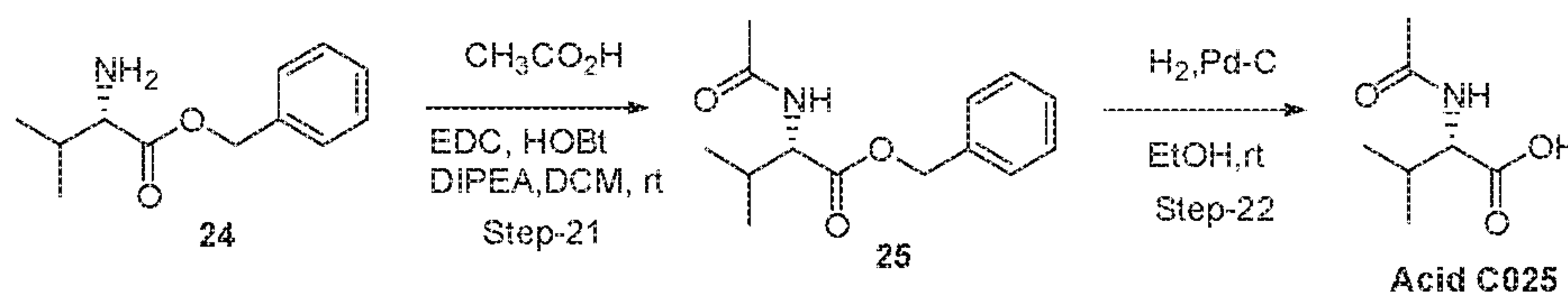
Scheme-4 [Synthesis of Acid C025]:
