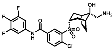
Intermediate 3
