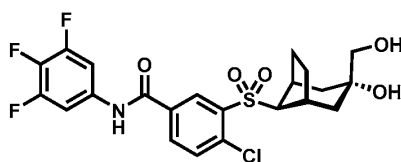
Intermediate 4
