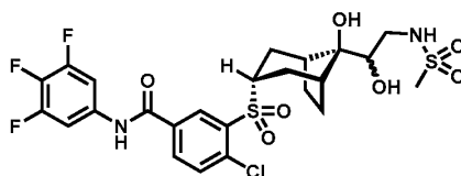
Example 26
