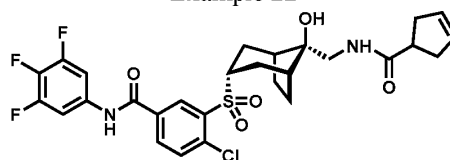
Example 22
