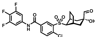
Intermediate 5
