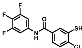
Intermediate 1
