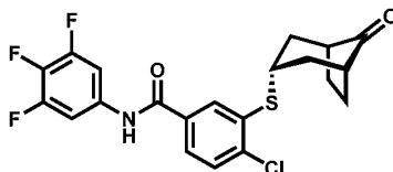
Intermediate 2
