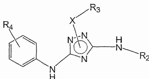
Formula (Ib)
