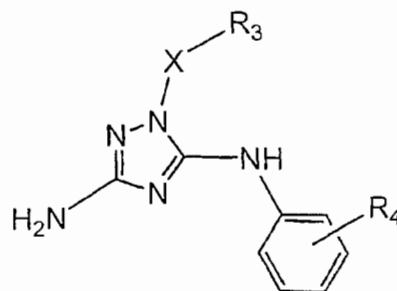
Formula (Id)
