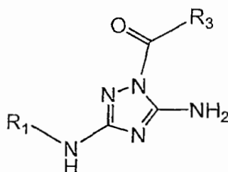
Formula (Ie)
