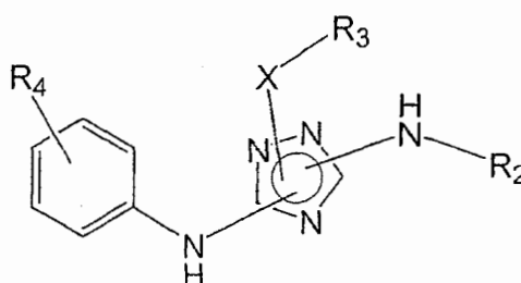
Formula (Ia)
