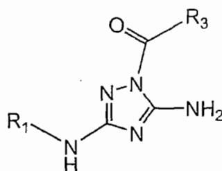
Formula (Ie)
