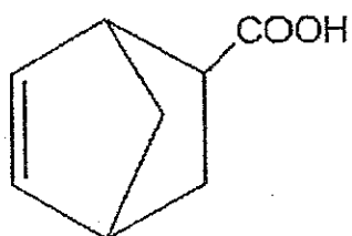
..... Compound A-1
