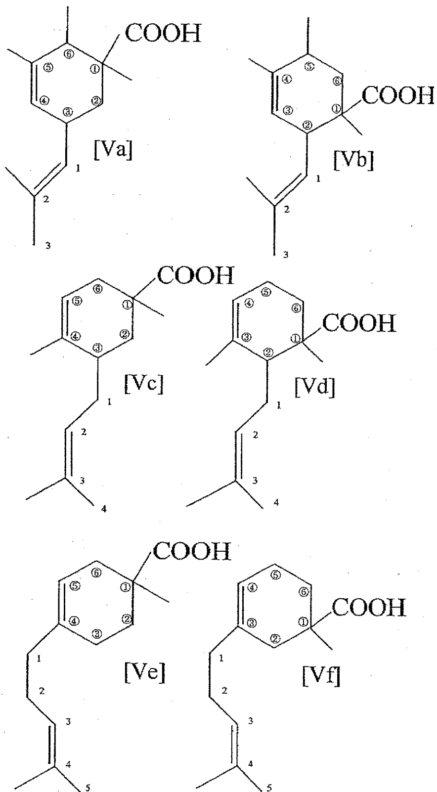
[Compound 4]
