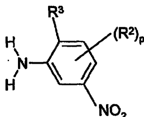
Formula VI
