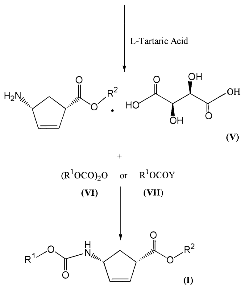
SCHEME 2
