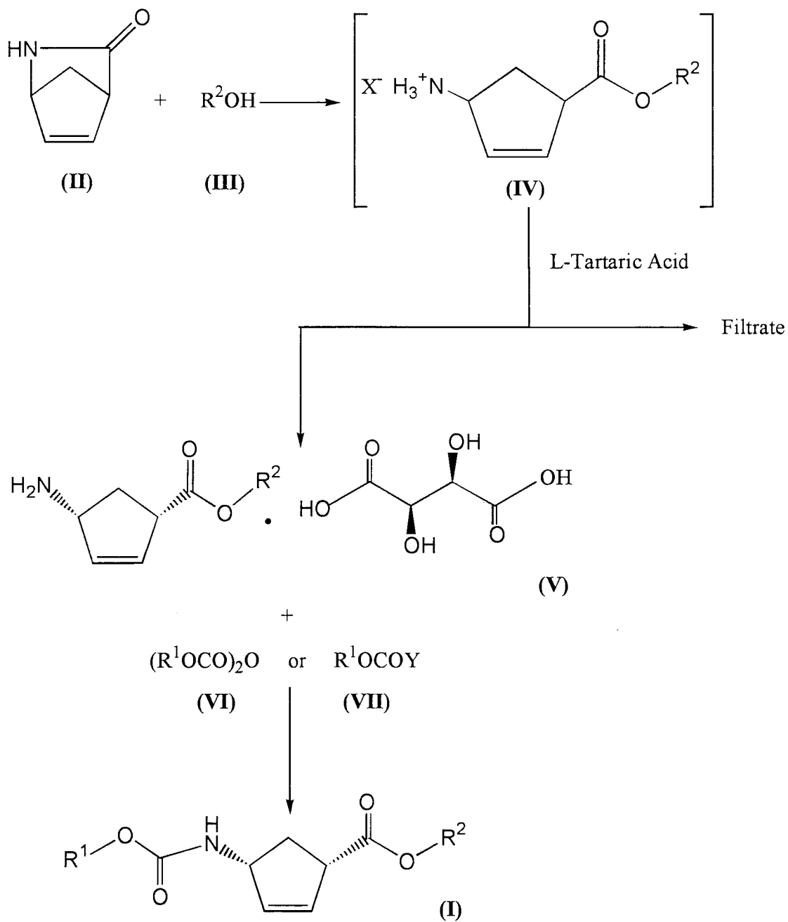
Scheme 1
