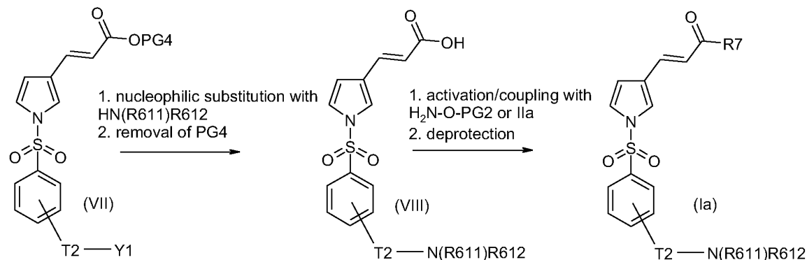
Reaction scheme 2:
