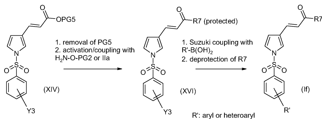
Reaction scheme 7:
