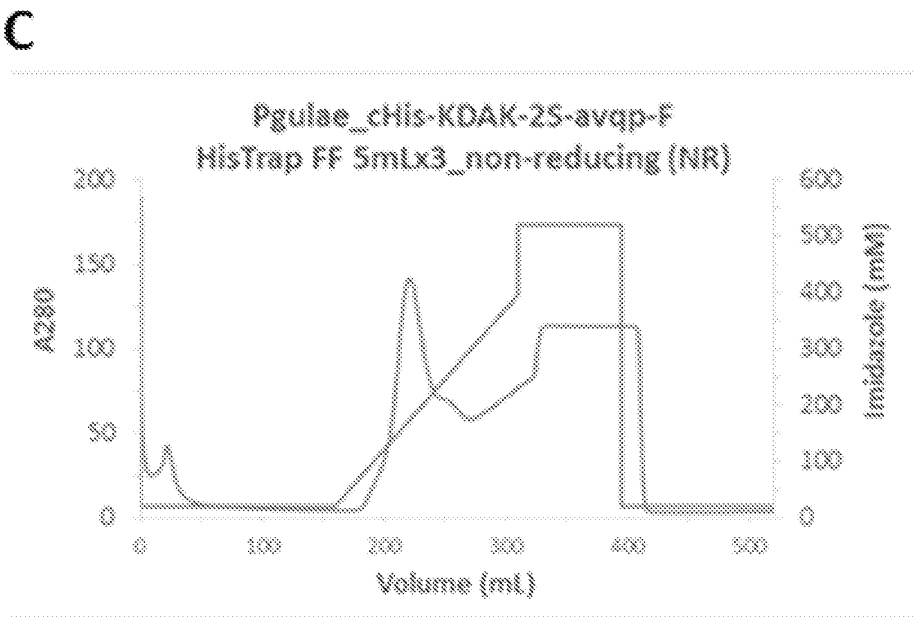
Ni-affinity chromatogram
