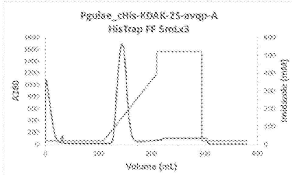
Ni-affinity chromatogram
