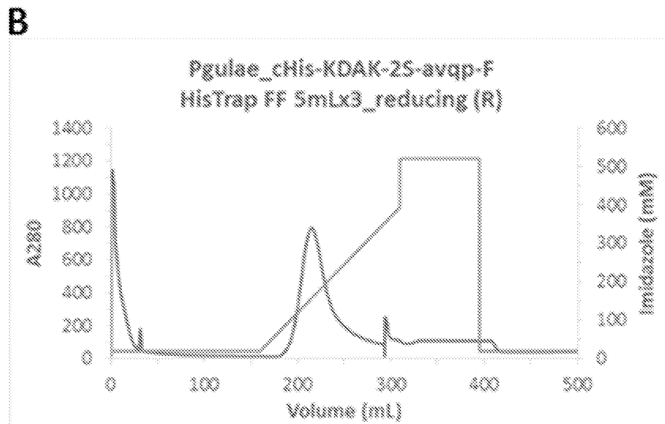
Ni-affinity chromatogram
