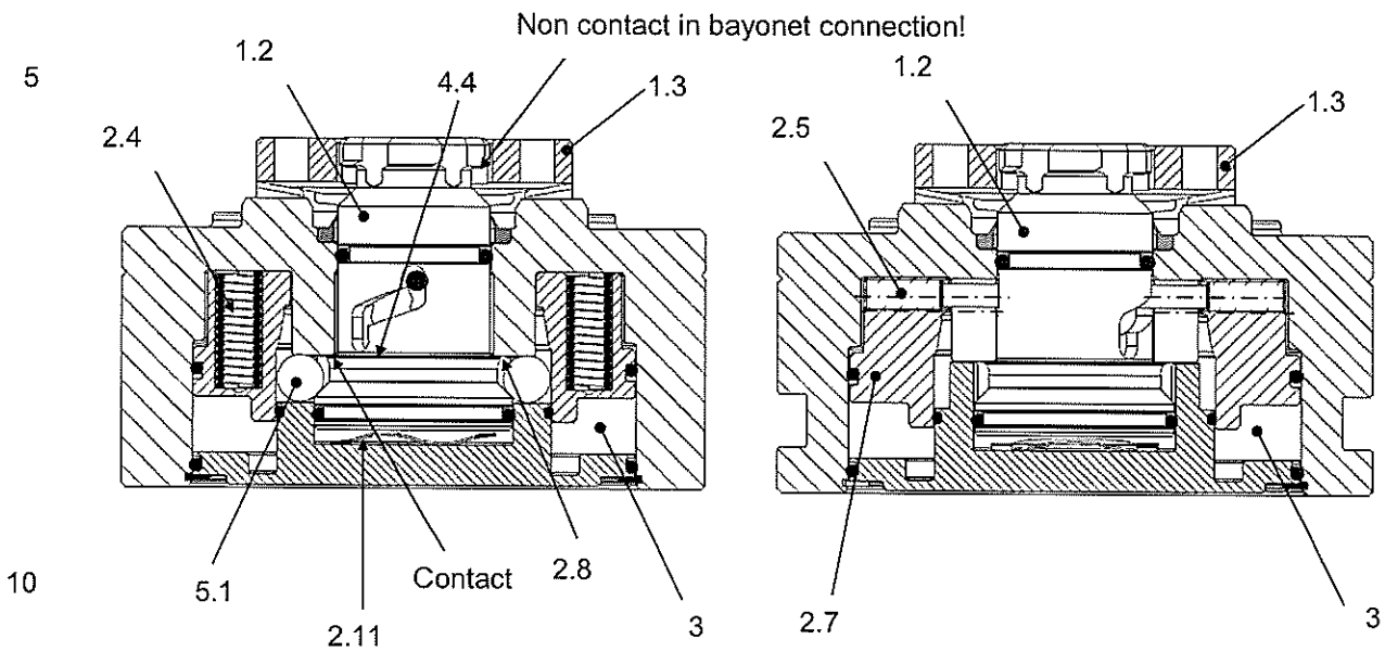
Fig 6a. Clamping chuck with drawbar in open position, cross section in 0 degree and 90 degree
