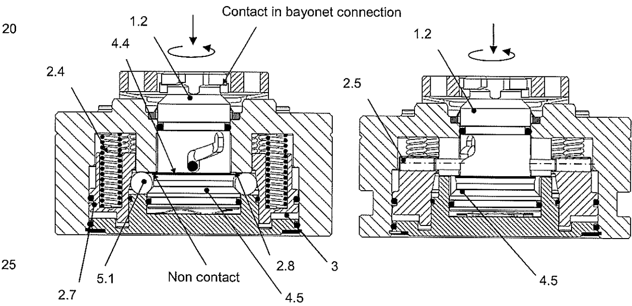
Fig 6b. Clamping chuck with drawbar in clamped position, cross section in 0 degree and 90 degree view
