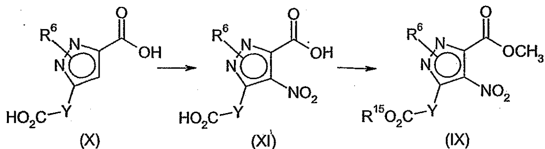
Scheme 11
