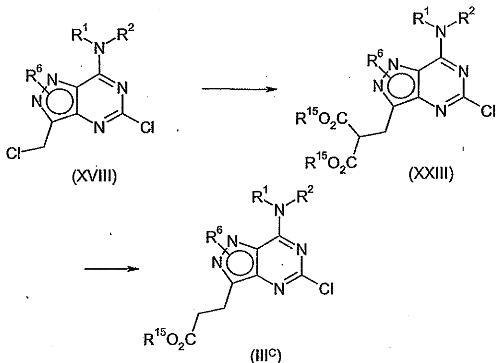
Scheme 24
