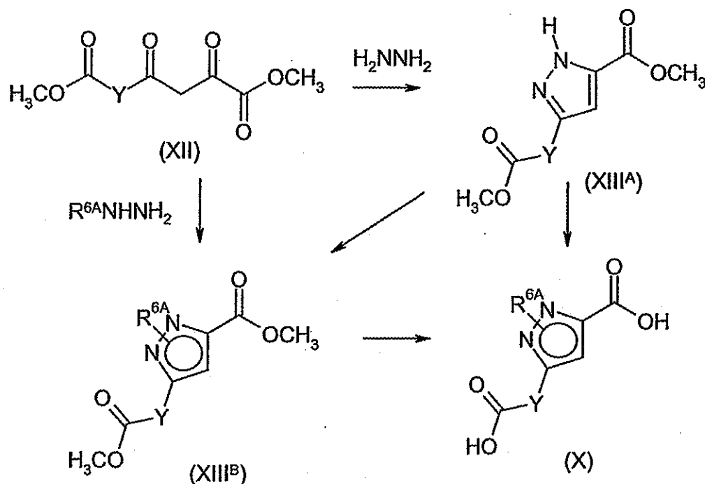
Scheme 12
