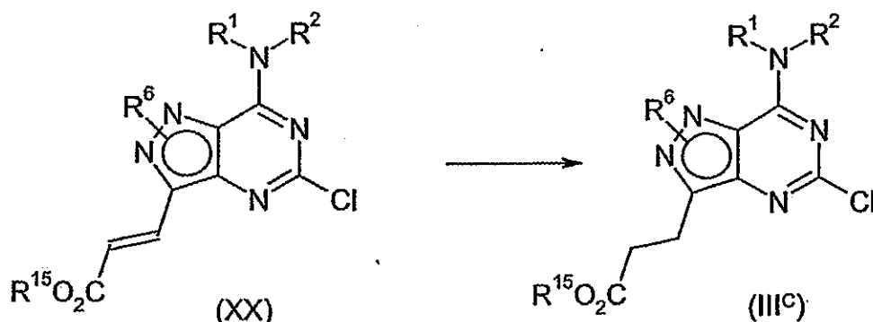
Scheme 20
