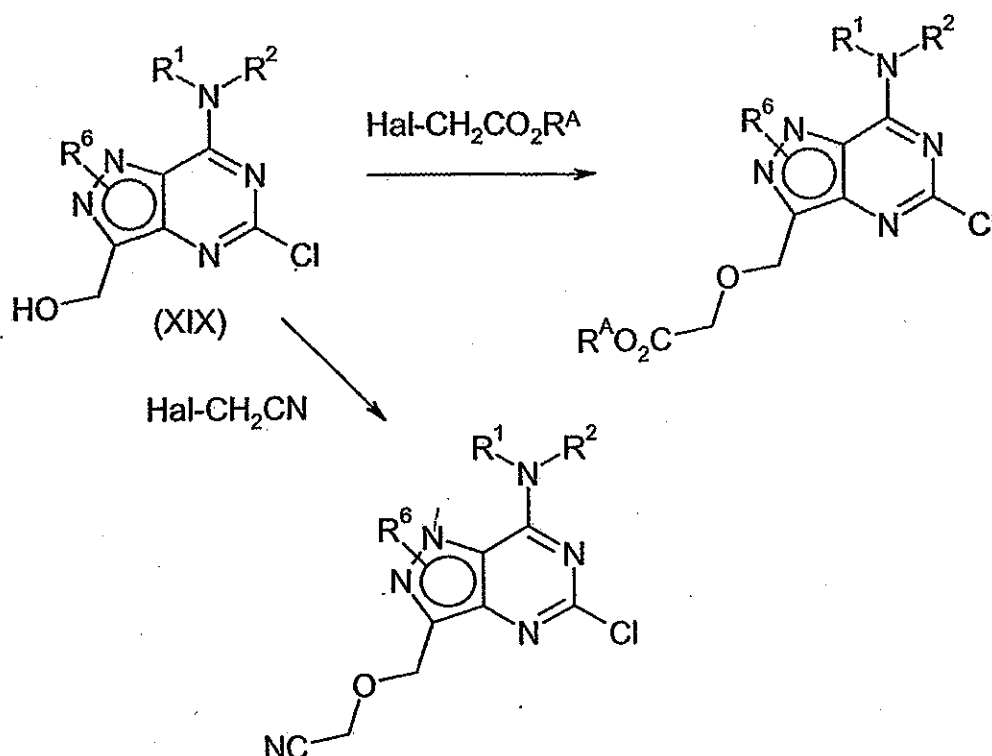
Scheme 30
