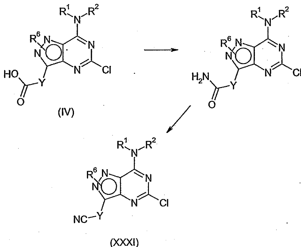
Scheme 29
