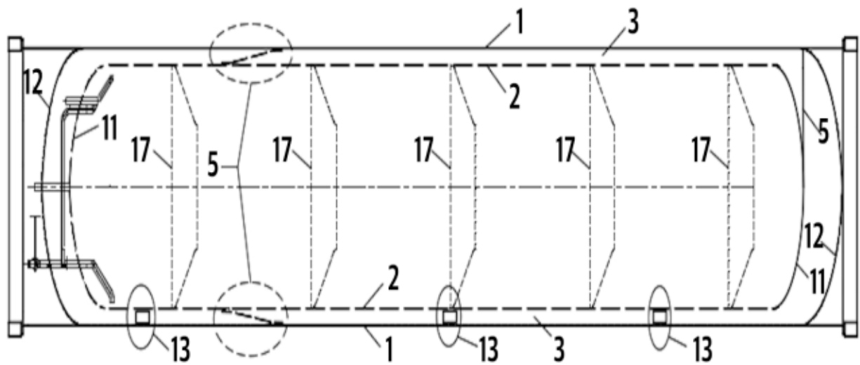
FIG. 1 - state of art vessel
