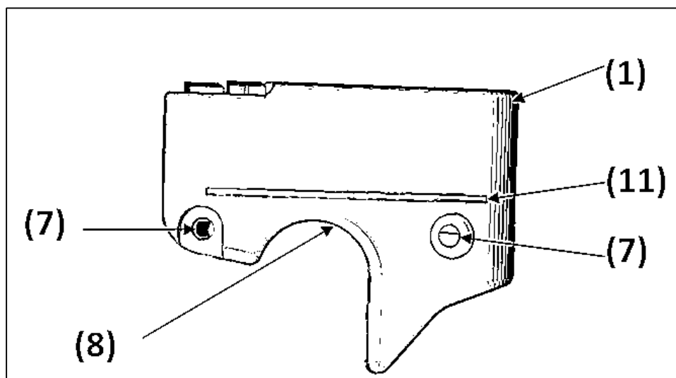
Figure 2-C Tibial template, front view
