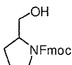
(a) Synthesis of ( S )-(9H-fluoren-9-yl)methyl 2-(hydroxymethyl)pyrrolidine-1-carboxylate
