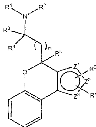
(VI),
