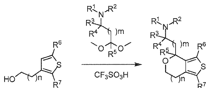
Scheme 2
