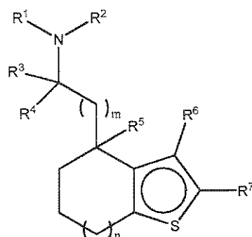
(IIc),
