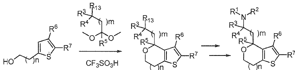
Scheme 7
