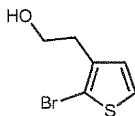
(a) Synthesis of 2-(2-bromothiophen-3-yl)ethanol
