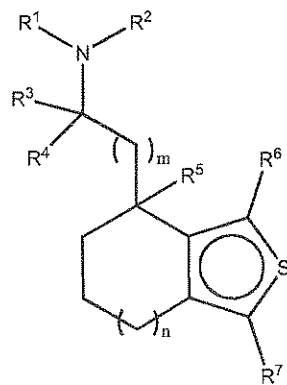
(IIIc),
