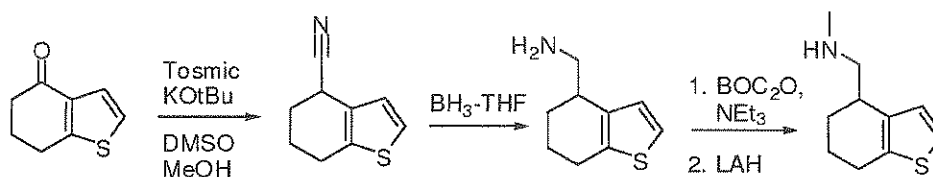
(a) Synthesis of 4,5,6,7-tetrahydrobenzo[b]thiophene-4-carbonitrile
