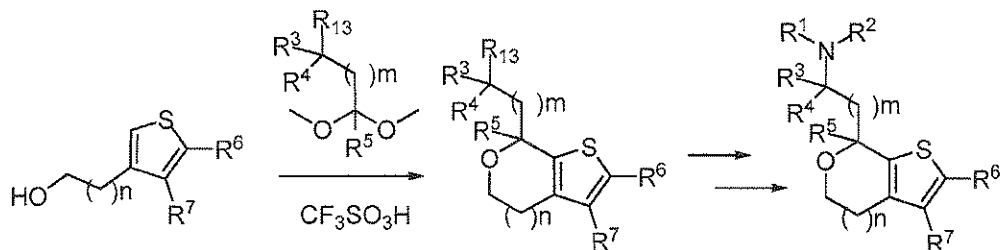
Scheme 9
