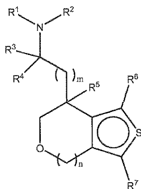
(IIIb),
