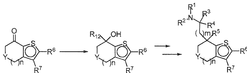
Scheme 6
