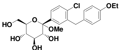
Compound B
