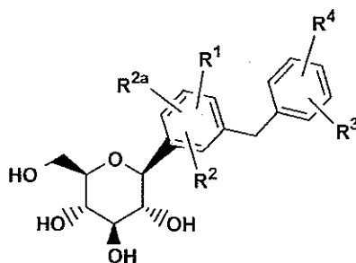
Compound D
