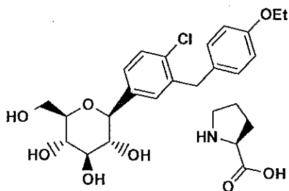
Compound Ii
