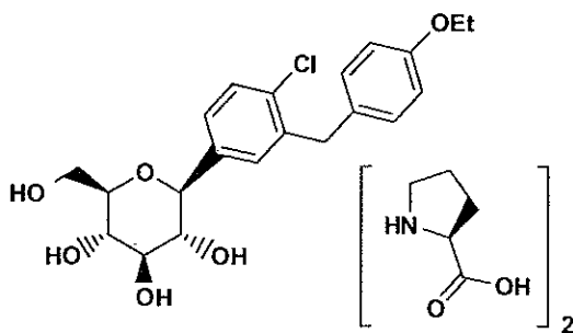
Compound Ih
