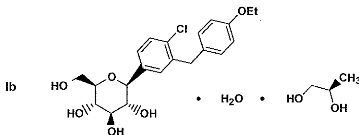
(R)-propylene glycol
