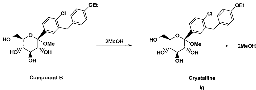
SCHEME V
