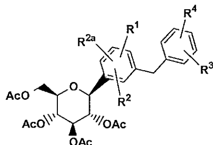
Compound C
