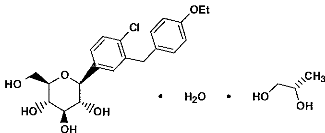
Compound Ia
