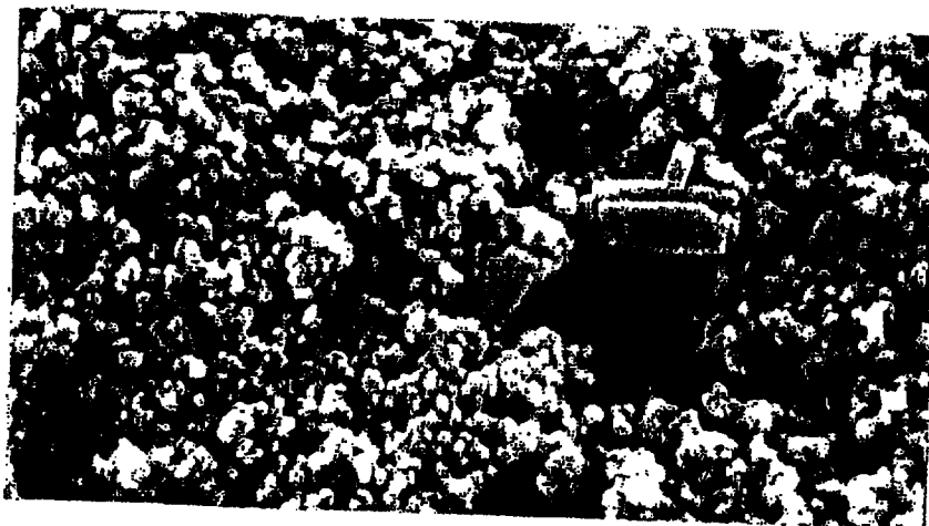
FIG.9 40,000 * SEM MICROGRAPH 1 HOUR AT 150 °C FORMATION OF THE FIRST CRYSTALS
