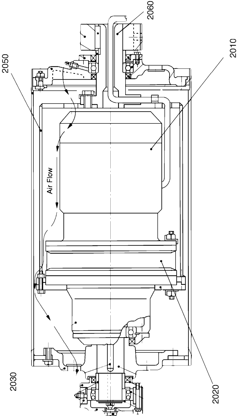
Fig. 2 Prior Art
