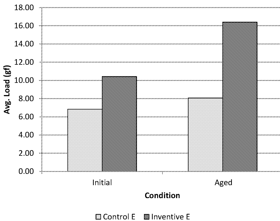
Figure 2. Peel Adhesion of Inventive Formulation “E” and Respective Control
