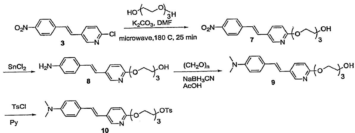
SCHEME 3
