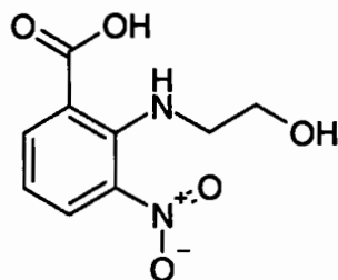
A. 2-[(2-Hydroxyethyl)amino]-3-nitrobenzoic acid
