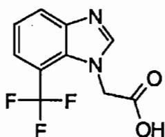
11) [7-(Trifluoromethyl)-1H-benzimidazol-1-yl]acetic acid
