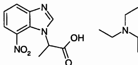
2) 2-(7-Nitro-1H-benzimidazol-1-yl)propanoic acid (triethylammonium salt)
