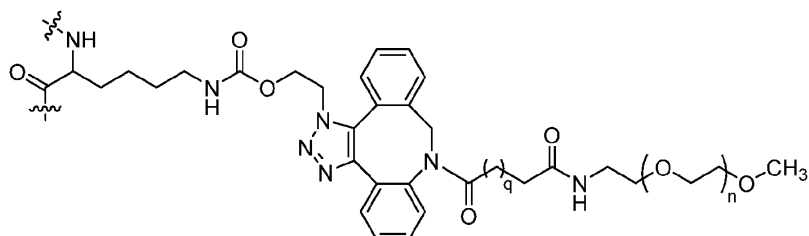
Formula (XIIA);
