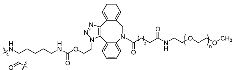
Formula (XIIIA);
