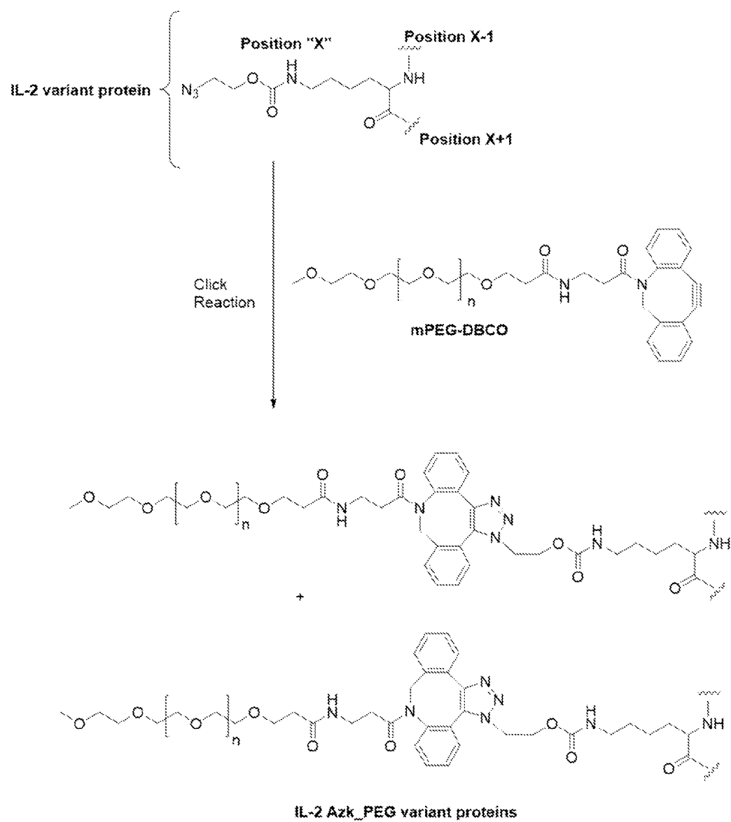
Scheme V.
