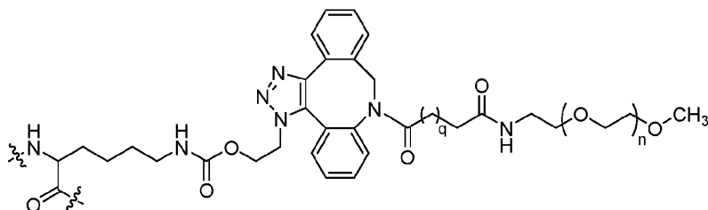
Formula (XIIIA);
