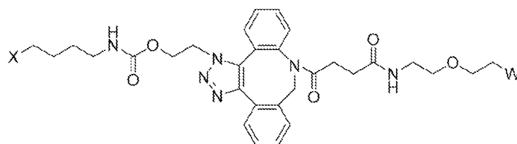
Formula (IV);
