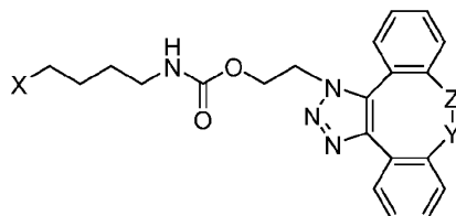
Formula (IA)
