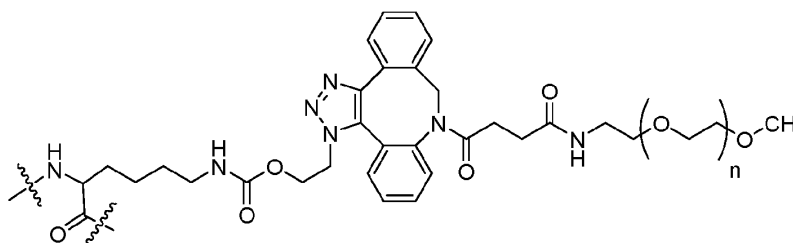
Formula (XII);
