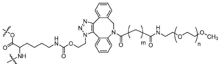
Formula (XVII);
