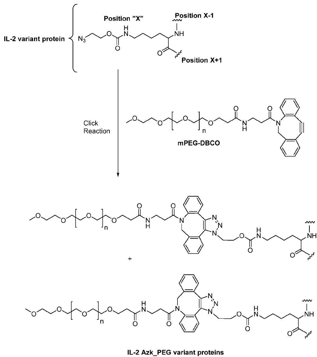
Scheme 1.
