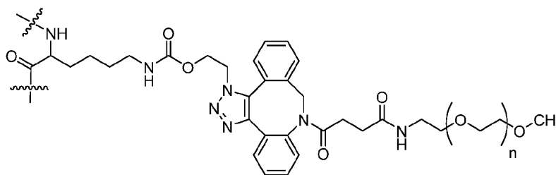
Formula (XII);
