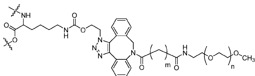
Formula (XVI);
