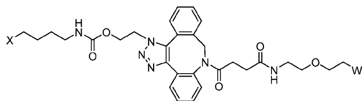
Formula (IV);
