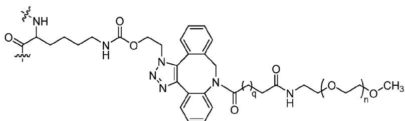
Formula (XIIA);
