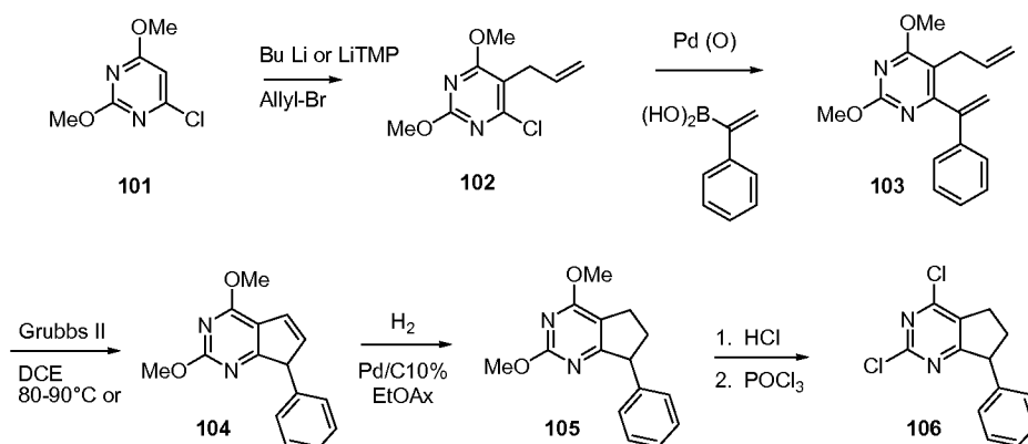
Scheme 23
