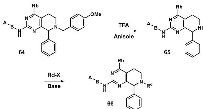
Scheme 16
