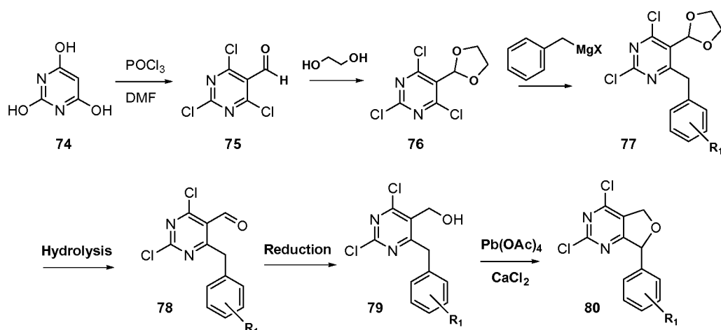
Scheme 18
