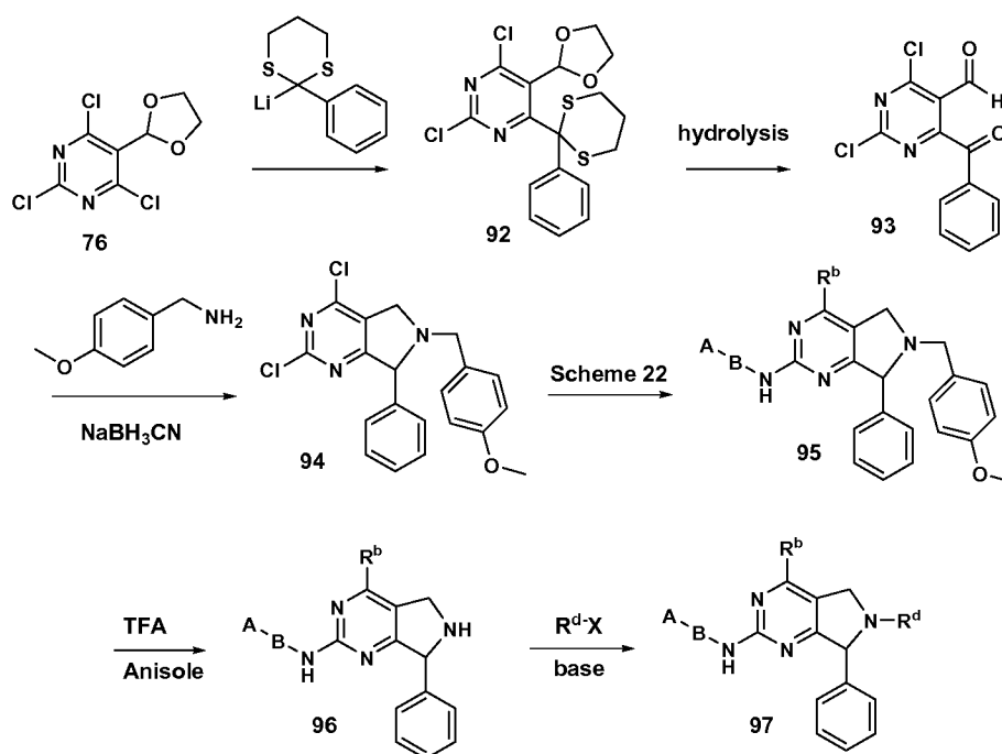
Scheme 21
