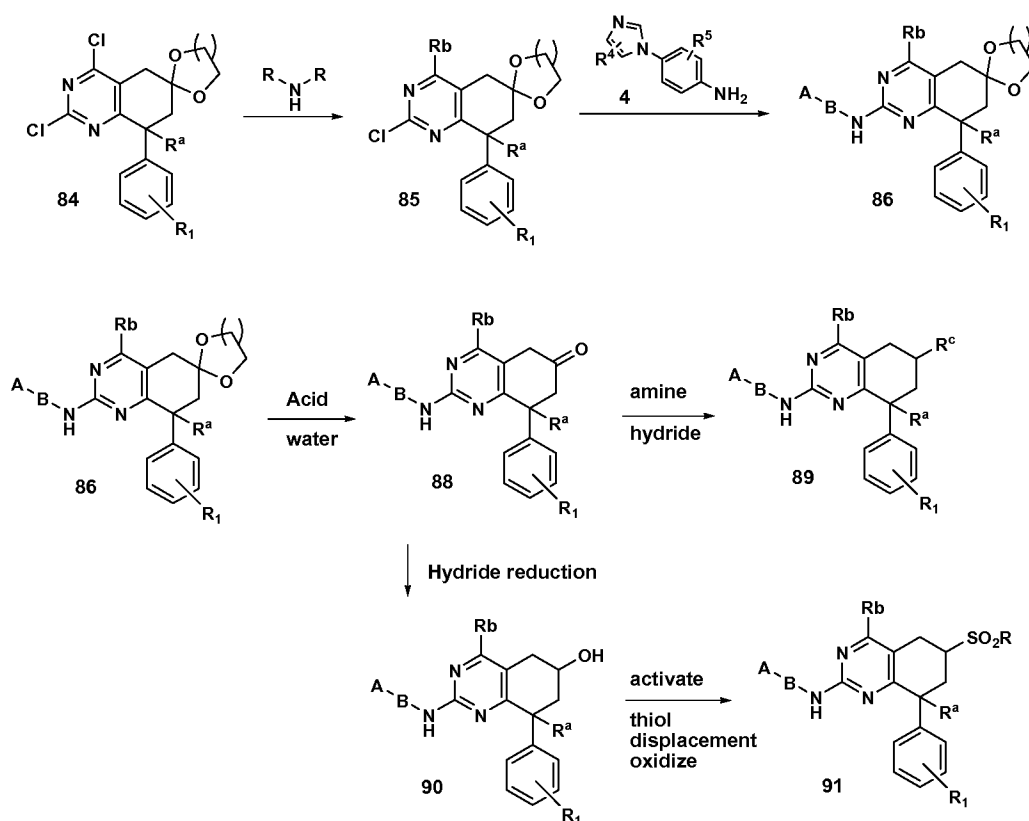
Scheme 20
