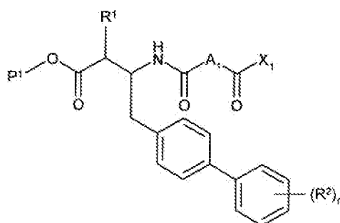
Intermediate C
