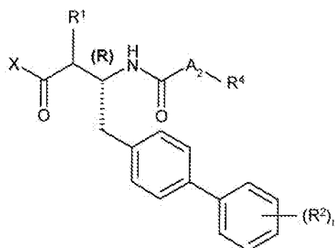
Formula VIIA
