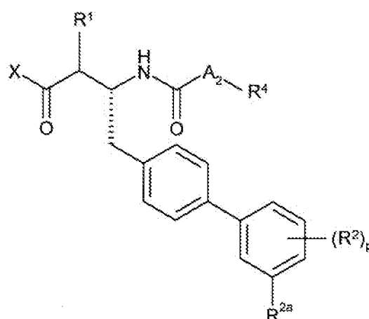
Formula VIIC
