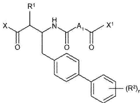
Formula II
