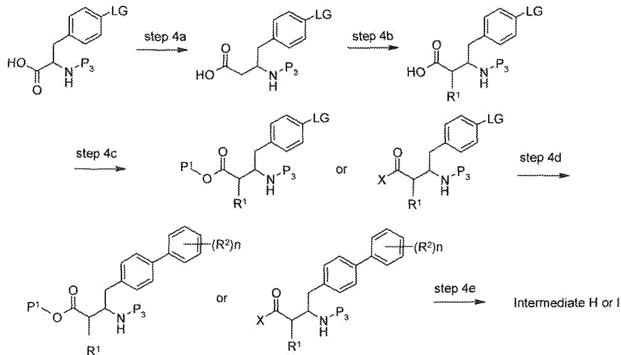
Scheme 4
