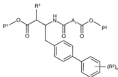
Intermediate A
