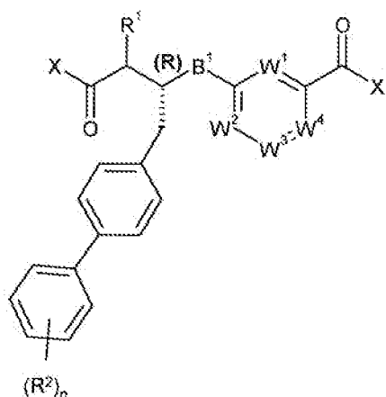
Formula VIA
