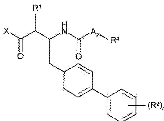
Formula VII
