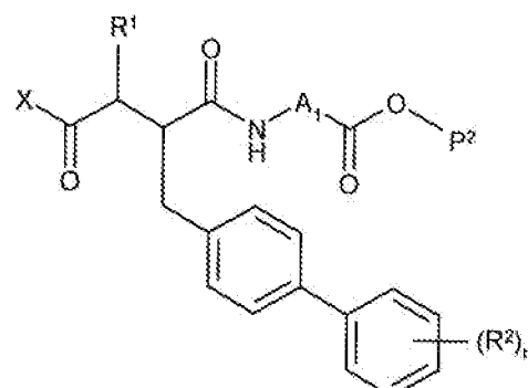
Intermediate E
