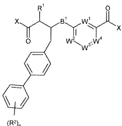
Formula VI
