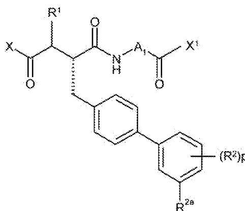
Formula IIIC
