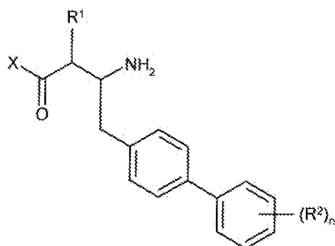
Intermediate H
