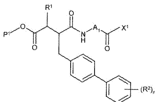
Intermediate F
