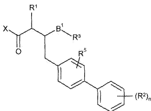
Formula I
