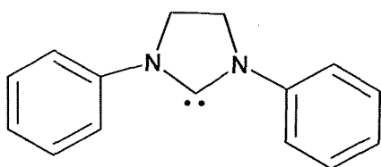
1,3-diphenyldihydroimidazol- 2-ylidene
