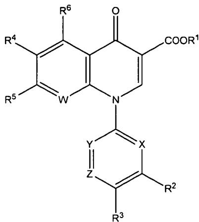
Pyridonecarboxylic Acid Derivative 1
