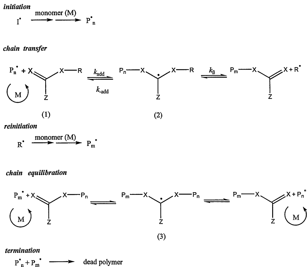
Scheme 1. Proposed mechanism of RAFT polymerisation
