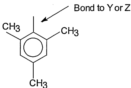
Formula 2
