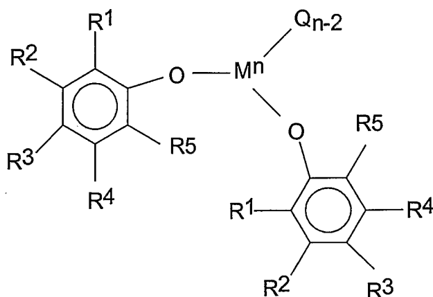
Formula (VIII)
