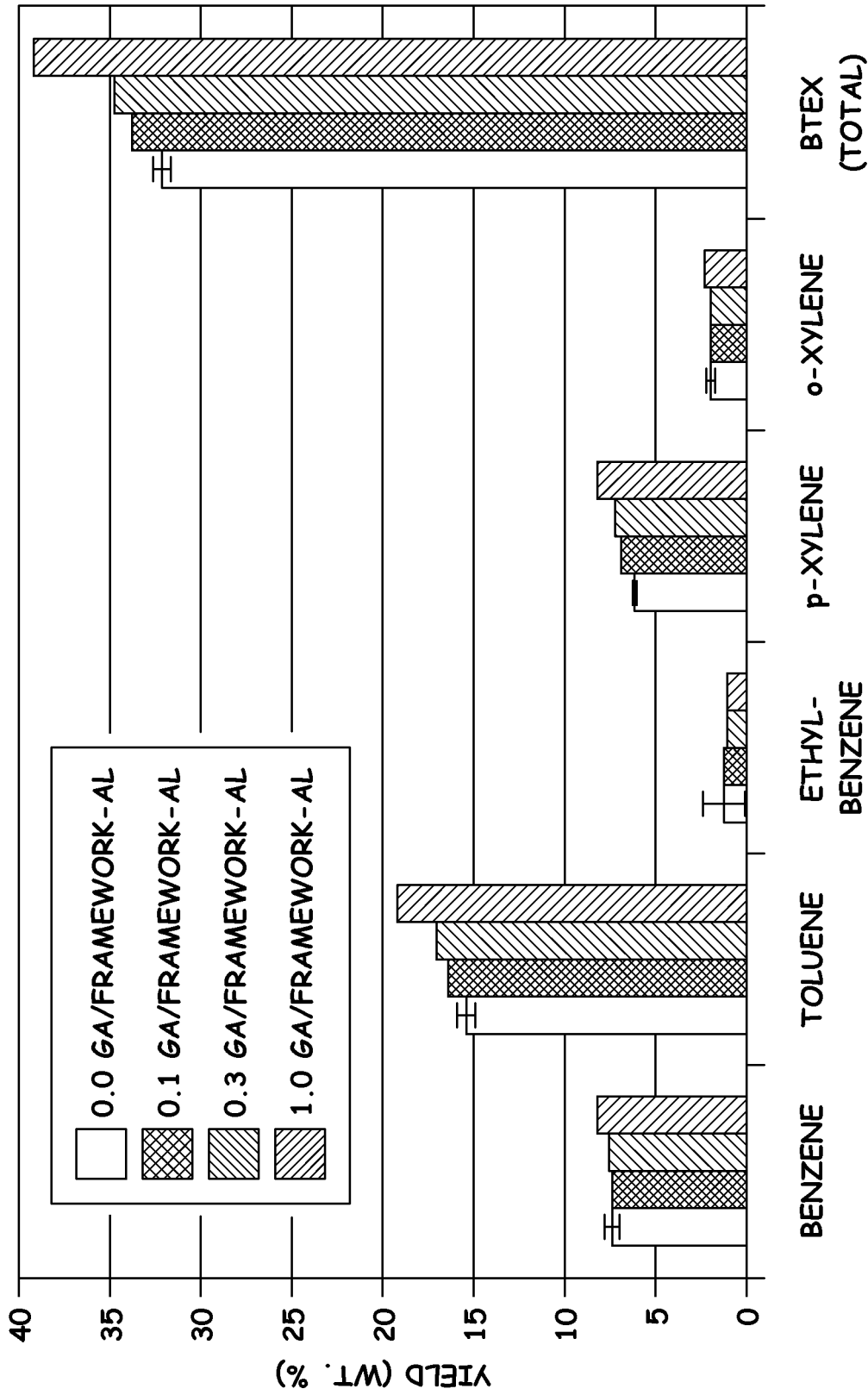
Fig. 6 (CANOLA OIL)
