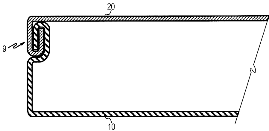
FIG. 3 (PRIOR ART)
