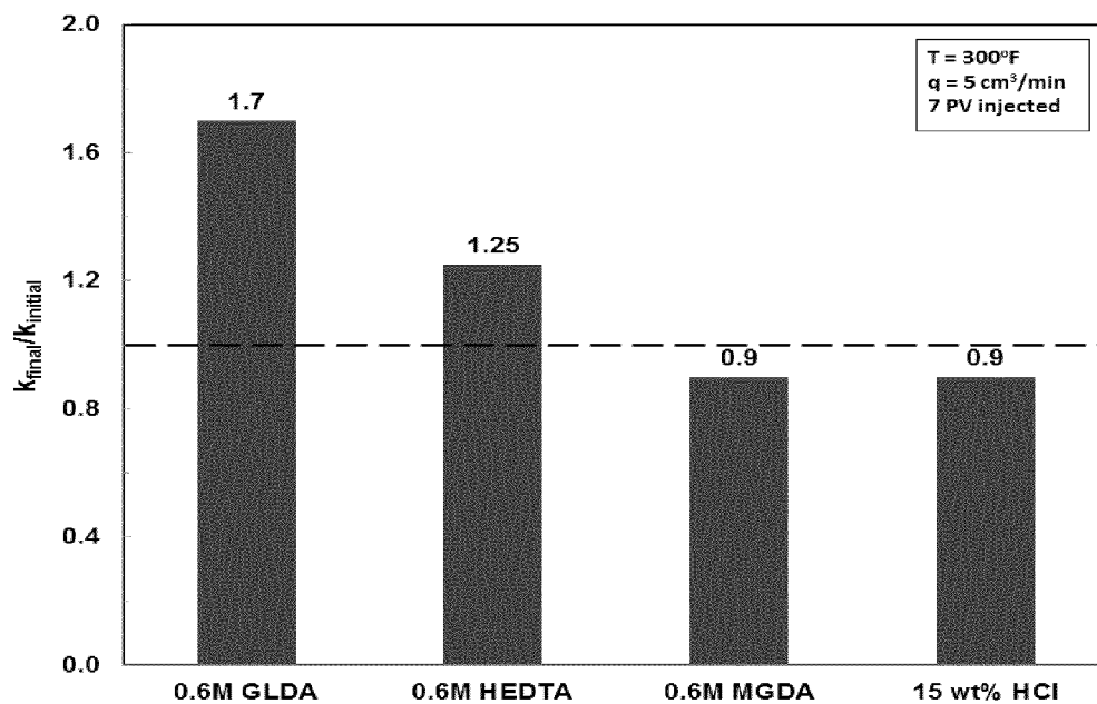
Fig. 3 - Permeability ratio for the Berea sandstone cores treated with 15 wt% HCl 5 and 0.6M chelating agent (pH =4) at 300°F and 5 cm 3 /min.
