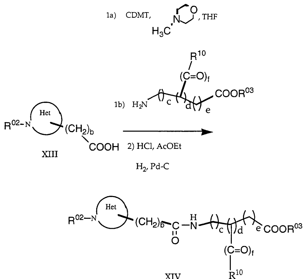
Scheme 3c
