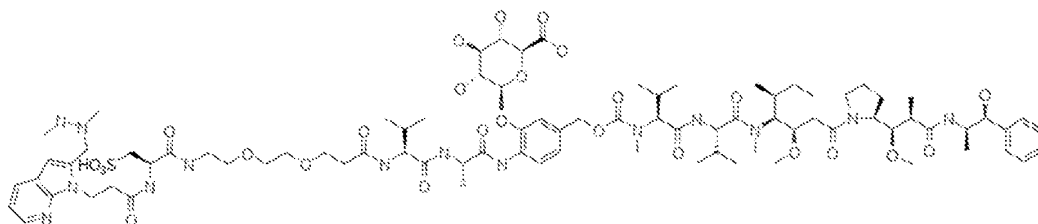
Vlb-82, Parent, C 84 H 130 N 14 O 26 S
