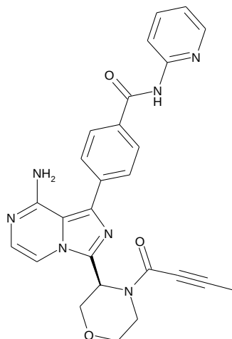
(R)-4-(8-Amino-3-(4-but-2-ynoylmorpholin-3-yl)imidazo[1,5-a]pyrazin-1-yl)-N-(pyridin-2-yl)benzamide
