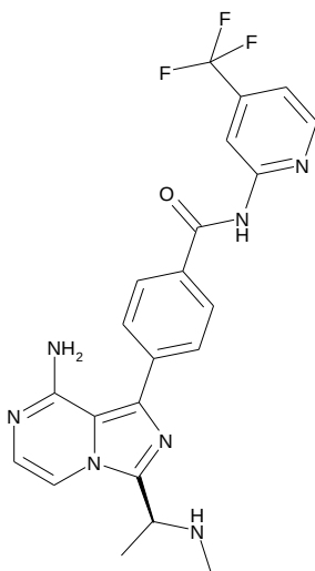
(S)-4-(8-Amino-3-(1-(methylamino)ethyl)imidazo[1,5-a]pyrazin-1-yl)-N-(4-(trifluoromethyl)pyridin-2-yl)benzamide
