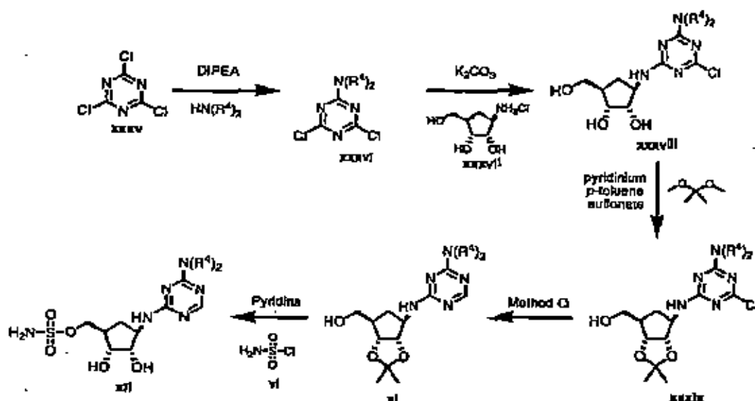
Scheme 5: Synthesis of ((1R,2R,3S,4R)-4-((4-((1S)-2,3-dihydro-1H-inden-1-ylamino)-1,3,5-triazin-2-yl)amino)-2,3-dihydroxycyclopentyl)methyl sulfamate
