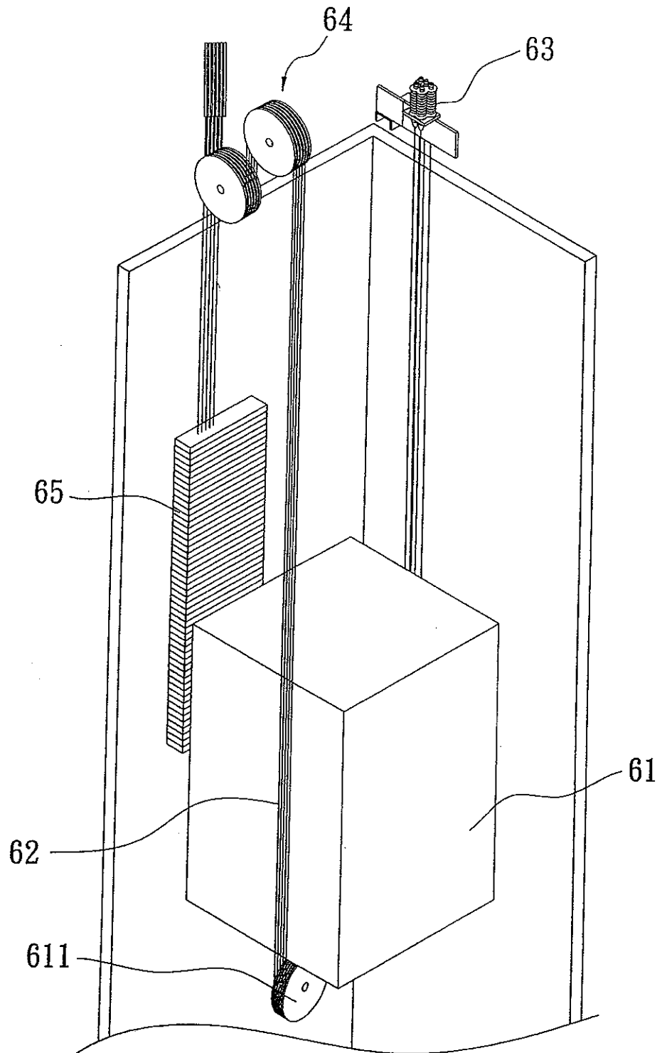
FIG. 7(PRIOR ART)
