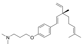
Compound 5
