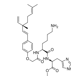
Compound 56
