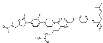
Compound 50
