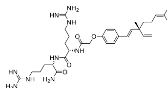
Compound 45
