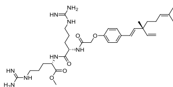
Compound 41
