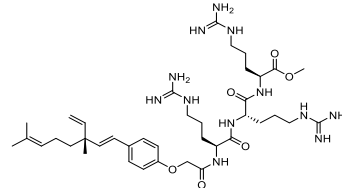
Compound 42
