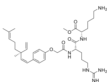
Compound 51
