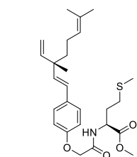
Compound 46
