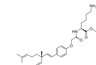
Compound 47
