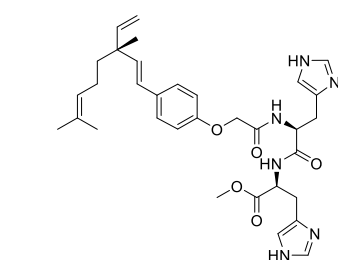
Compound 55
