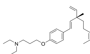
Compound 6
