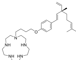
Compound 31
